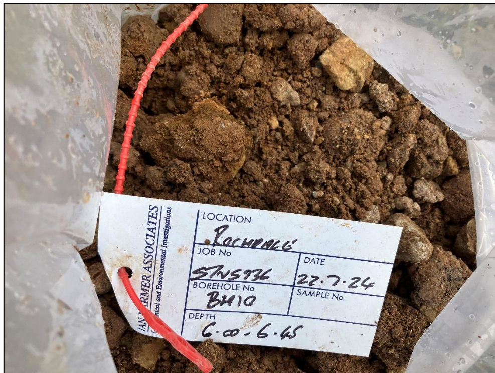
Photograph 28 – Photograph of the Hummocky Glacial Deposits between 6.0 – 6.45m depth bgl in BH10.
