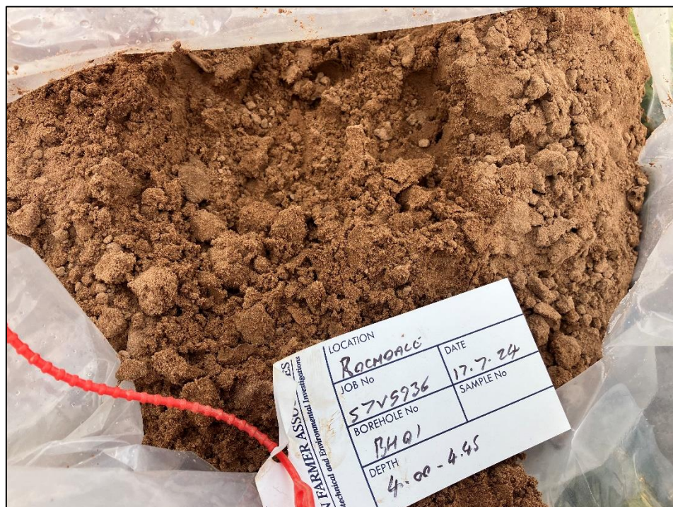
Photograph 2 – Photograph of the Hummocky Glacial Deposits between 4.0-4.45m bgl in BH01.
