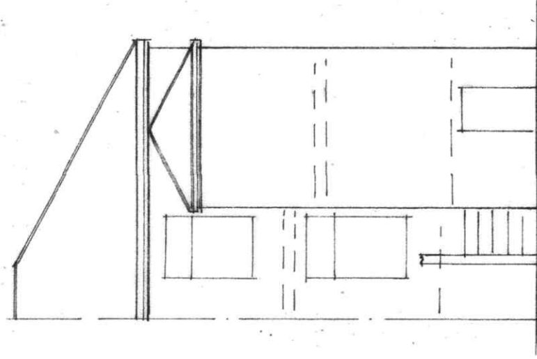
REAR ELEVATION (EXISTING)
