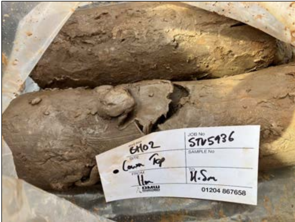
Photograph 7 – Photograph of Hummocky Glacial Deposits between 11.0 and 11.5m bgl in BH02.
