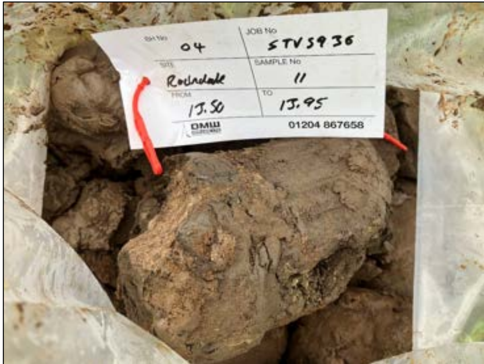
Photograph 13 – Photograph of the Hummocky Glacial Deposits between 13.5 and 13.95m depth bgl in BH04.
