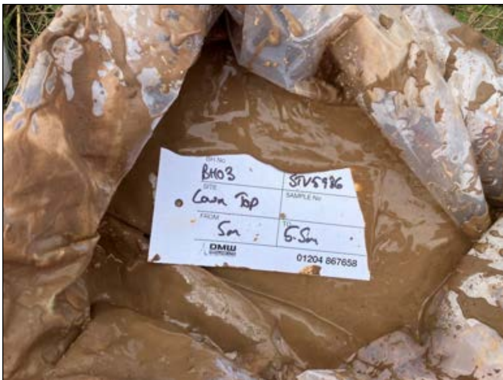
Photograph 10 – Photograph of the Hummocky Glacial Deposits between 5.0 – 5.5m bgl in BH03.
