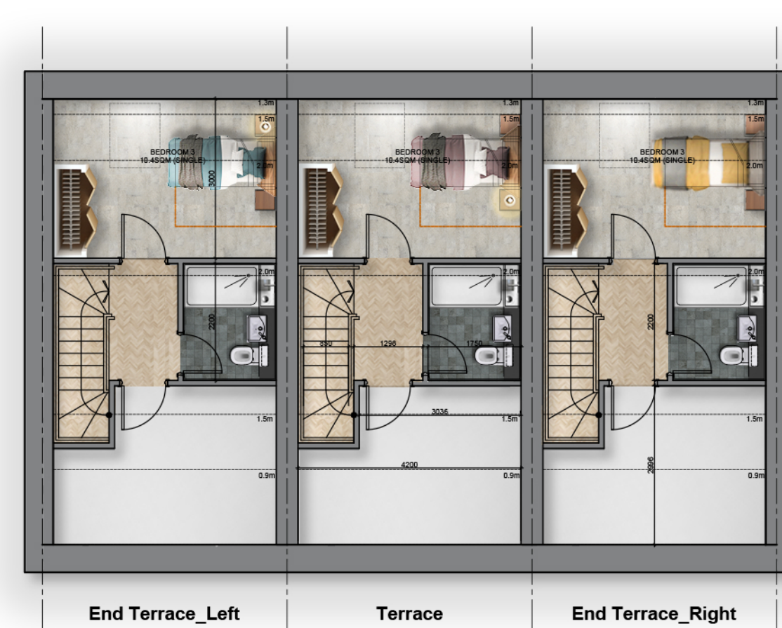
3 BED 4P - SECOND FLOOR Floor Area: 21.48 sq.m.
