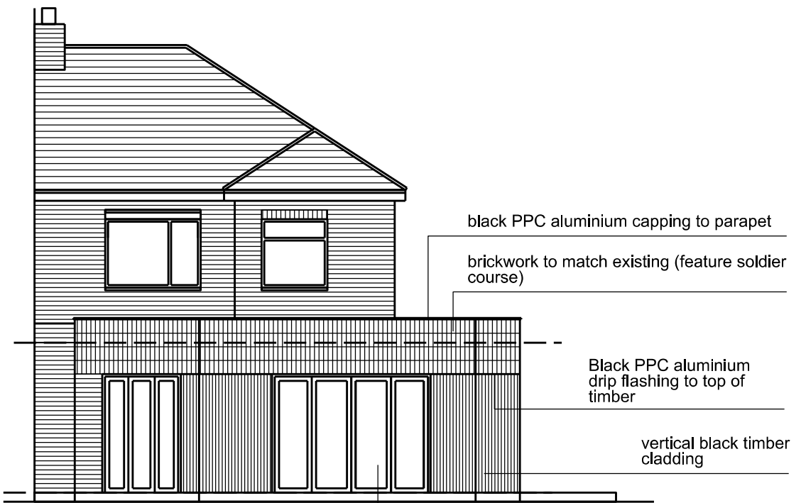
West Elevation
