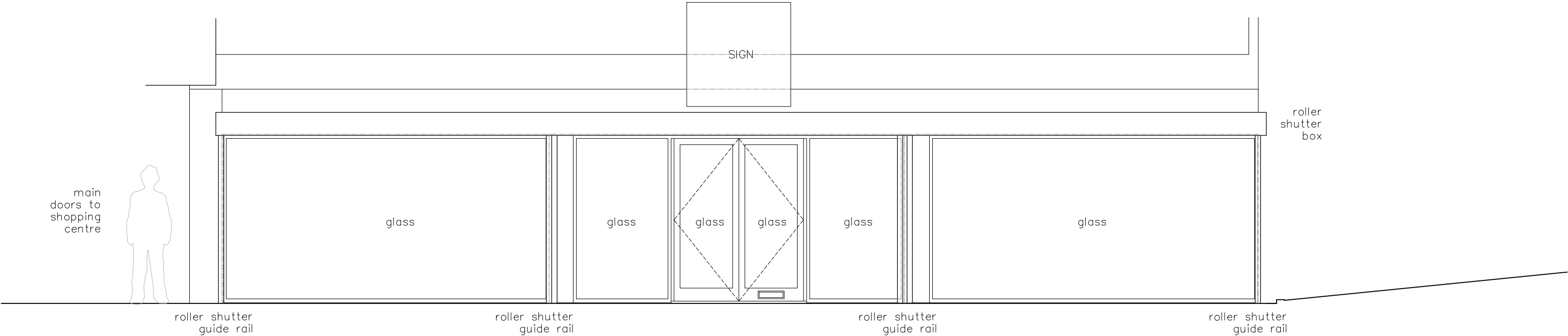
External Middleton Gardens Elevation (shutters up)
