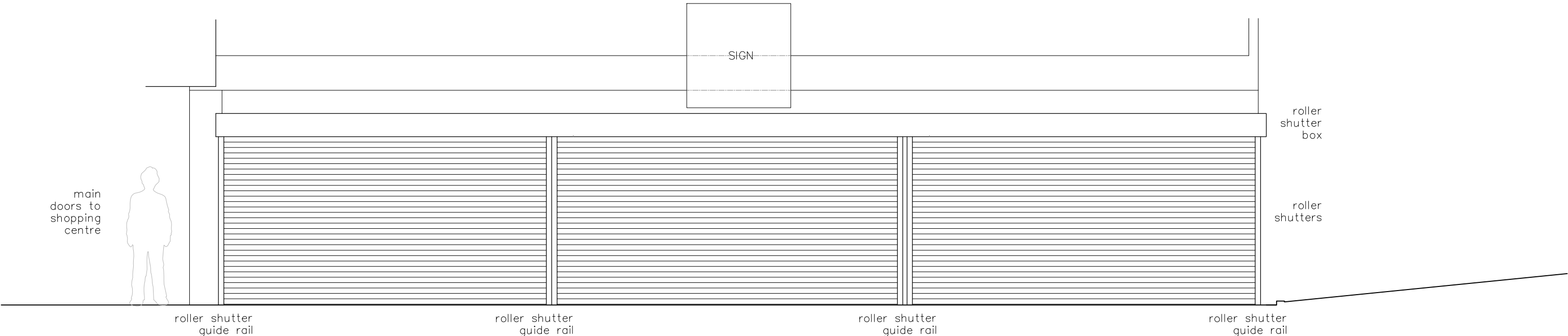
External Middleton Gardens Elevation (shutters down)
