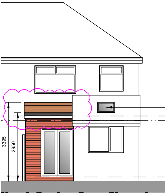
North Facing Rear Elevation
