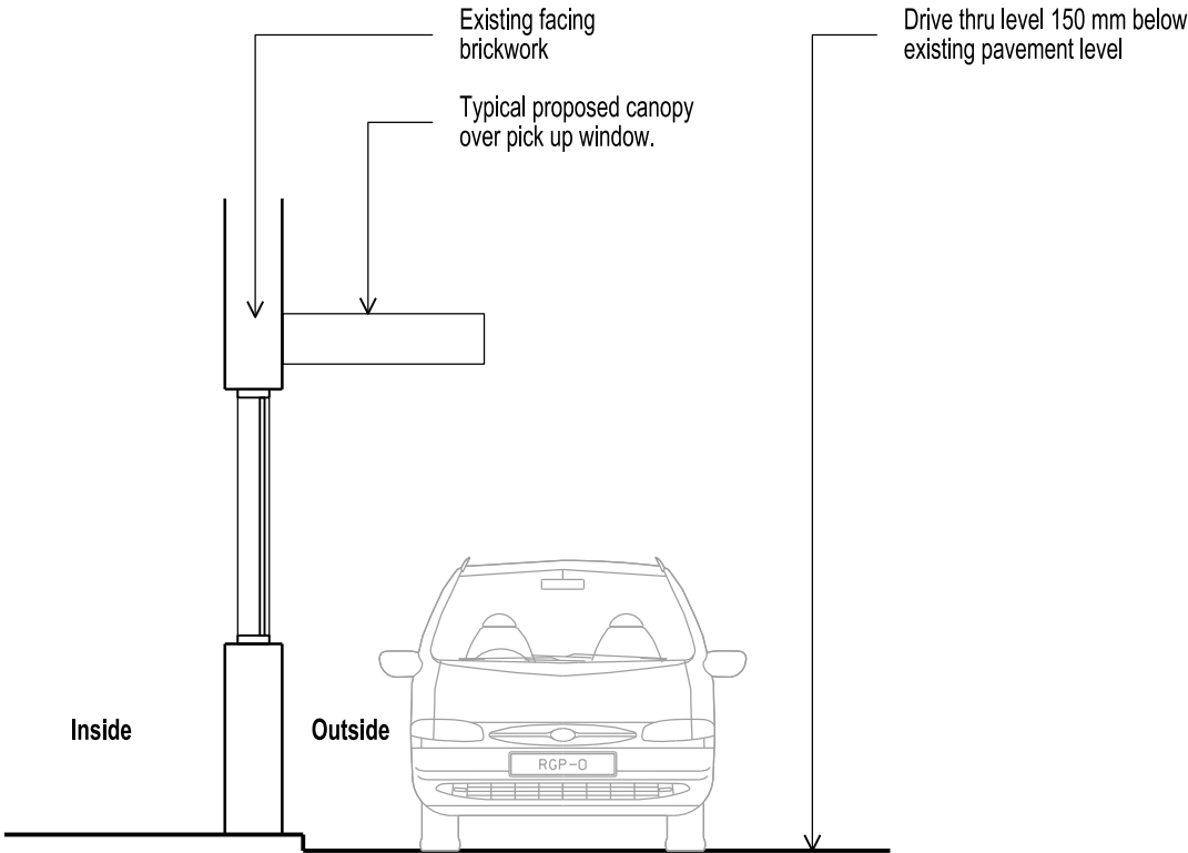
PROPOSED SECTION DETAIL
