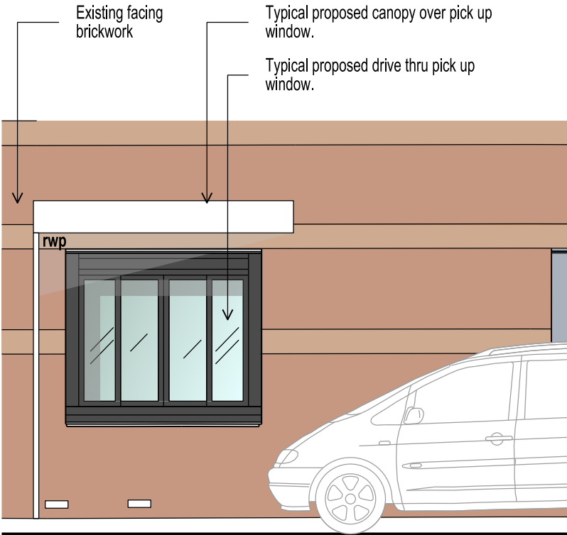
PROPOSED SOUTH -EAST ELEVATION
