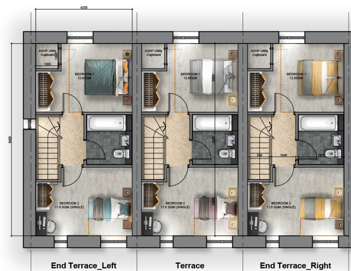
2 BED 3P - FIRST FLOOR Floor Area: 35.27 sq.m. Total Area: 70.54 sq.m (70 sq.m)
