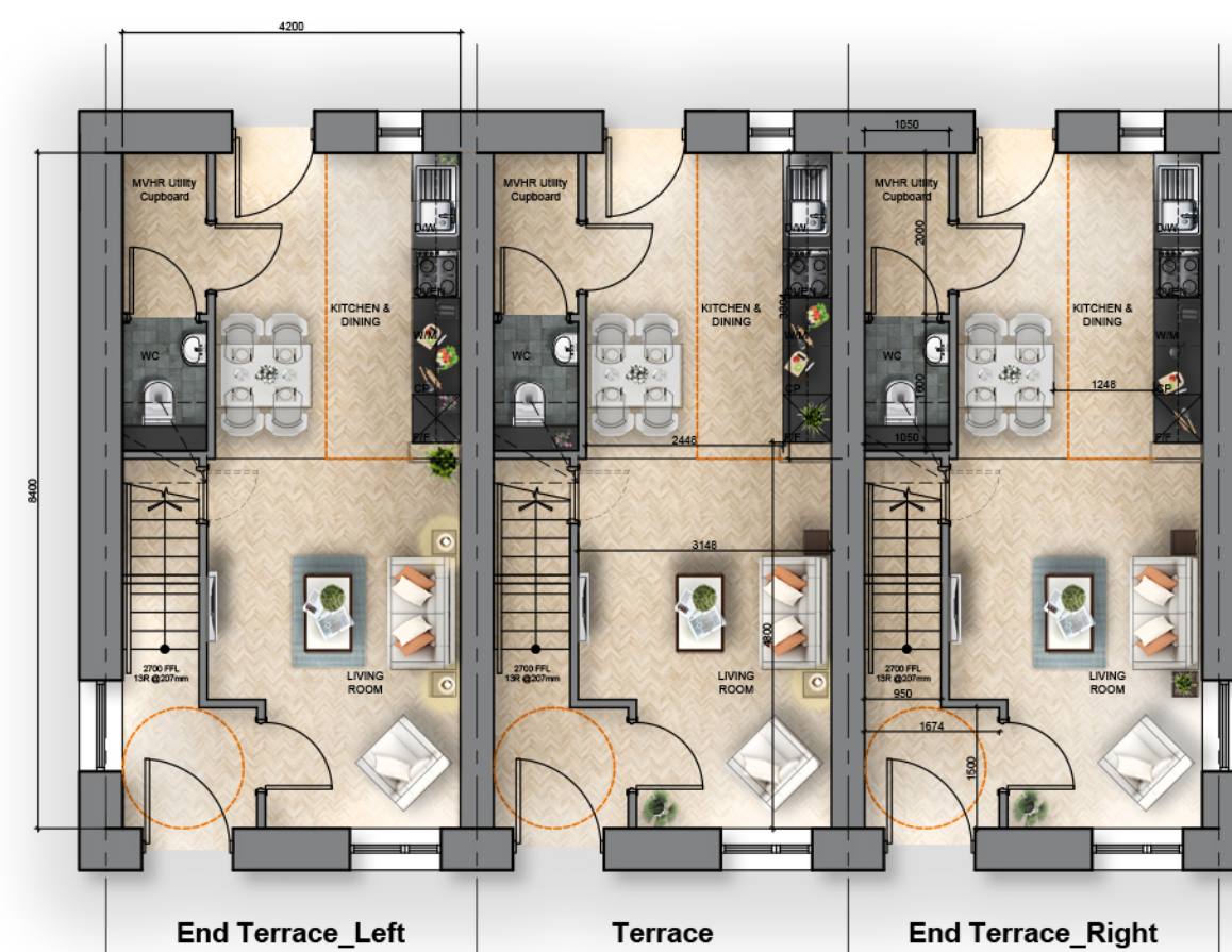
2 BED 3P - GROUND FLOOR Floor Area: 35.27 sq.m.
