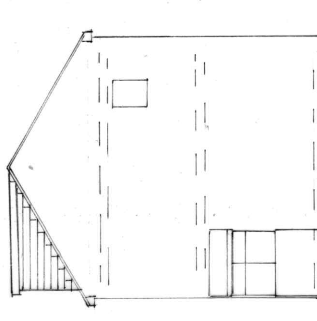
SIDE ELEVATION (PROPOSED)
