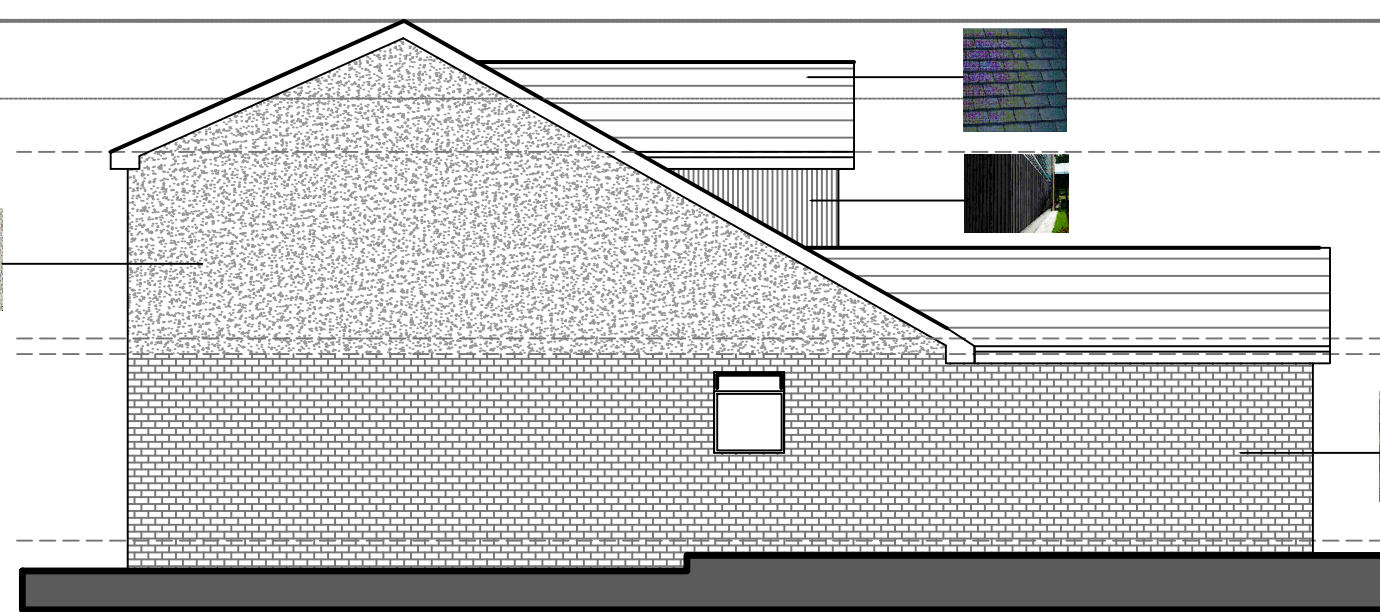
EPROPOSED SIDE ELEVATION 1:100
