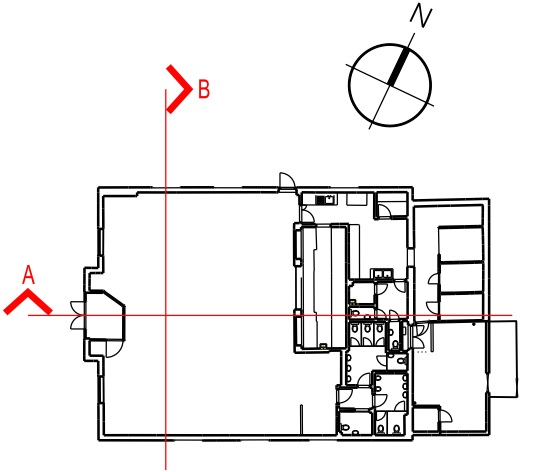
EXISTING GROUND FLOOR PLAN - nts
