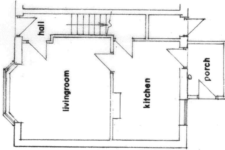
G.F. PLAN (EXISTING)
