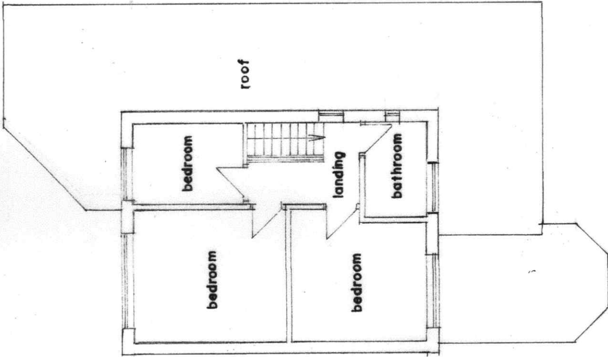
FIRST FLOOR PLAN (EXISTING)
