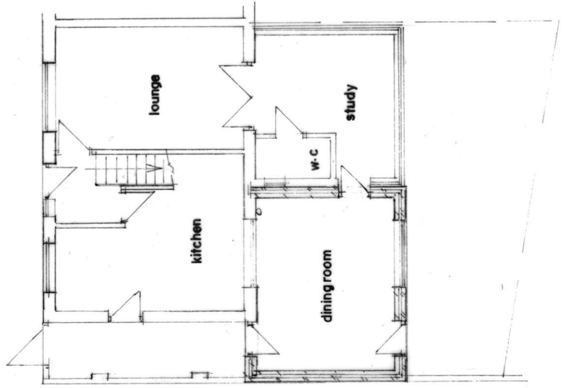
GROUND FLOOR PLAN (PROPOSED)
