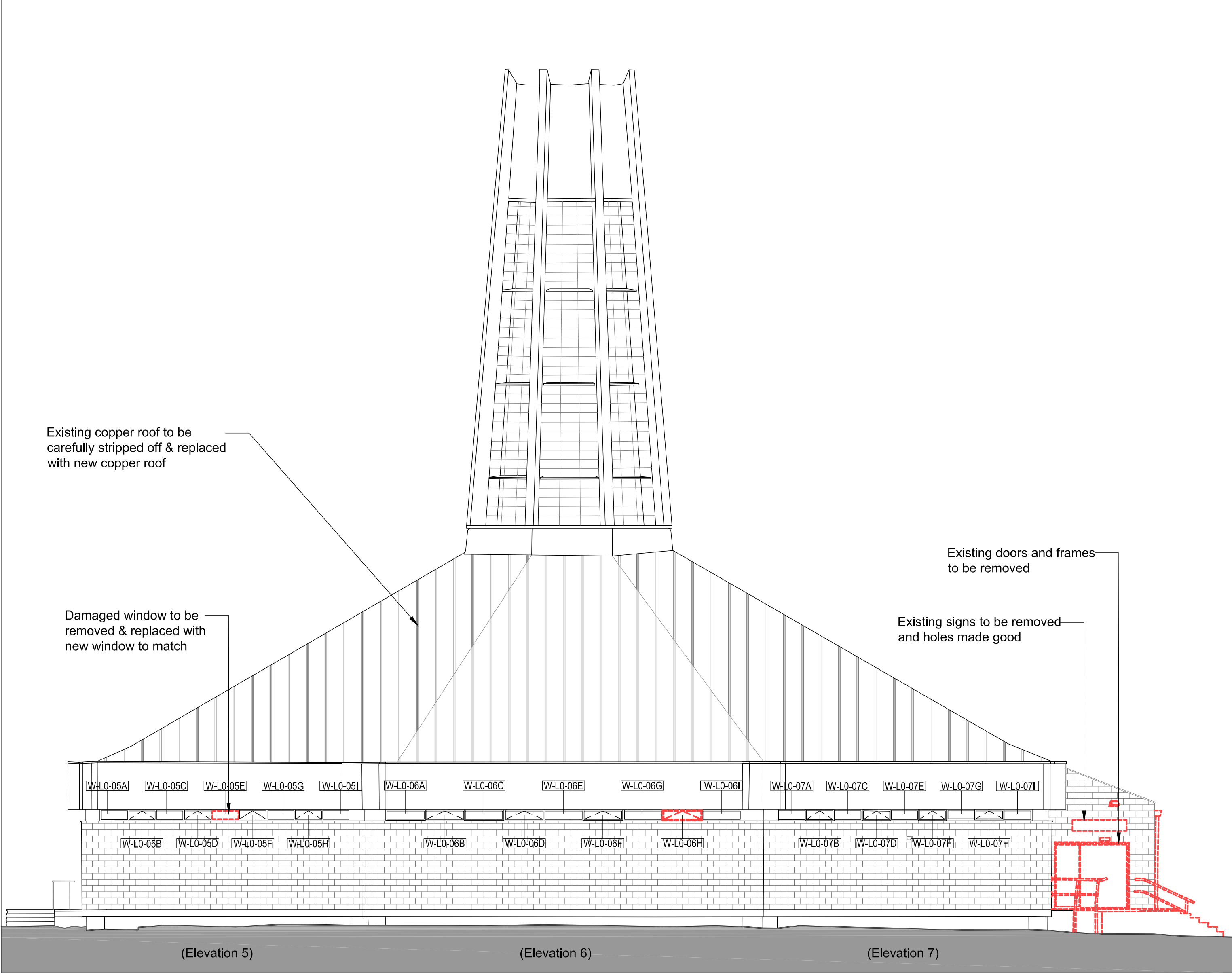
Existing Elevation C
