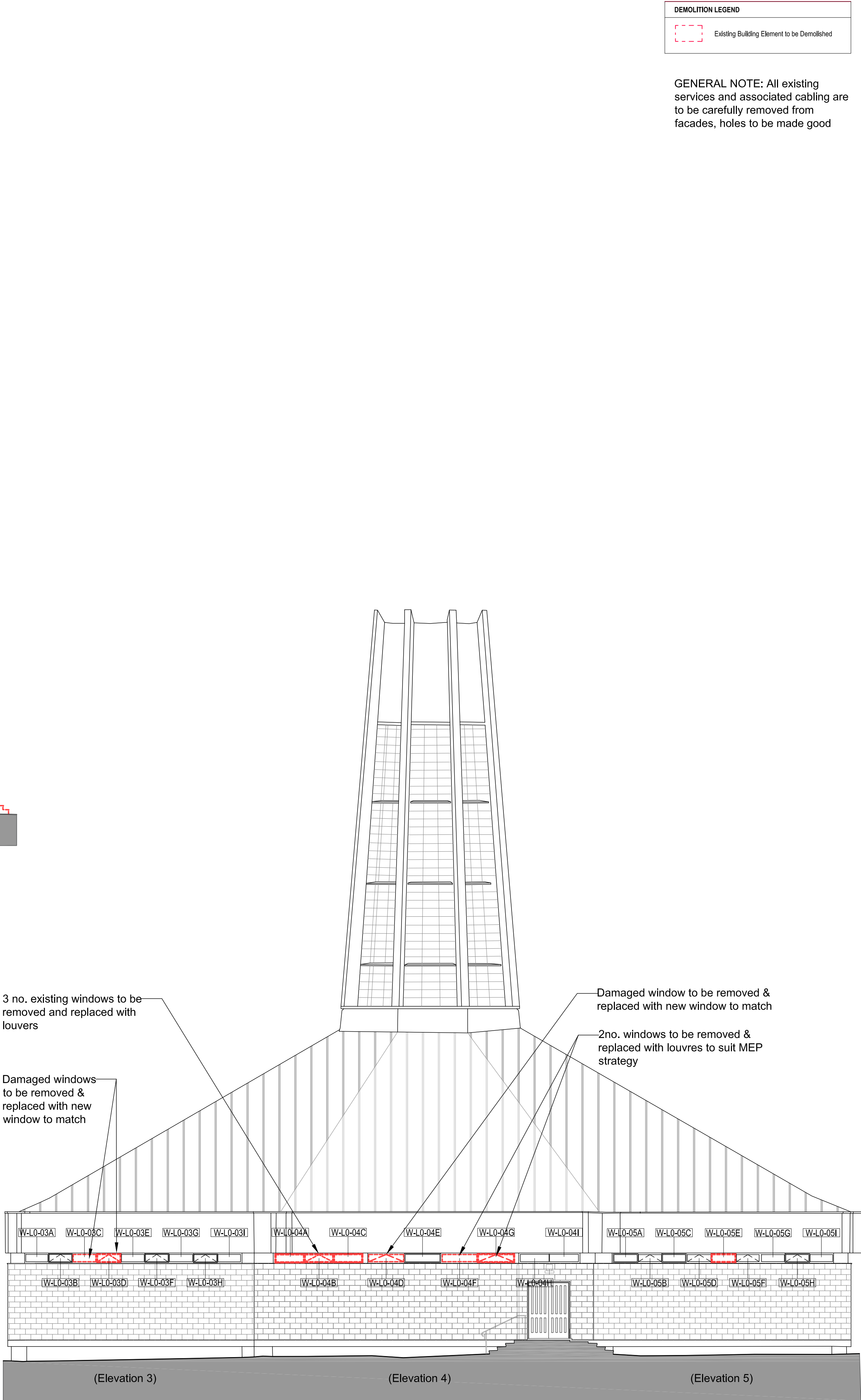
Existing Elevation D
