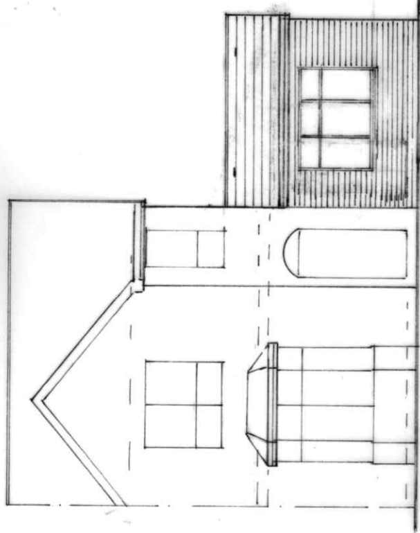
FRONT ELEVATION (PROPOSED)
