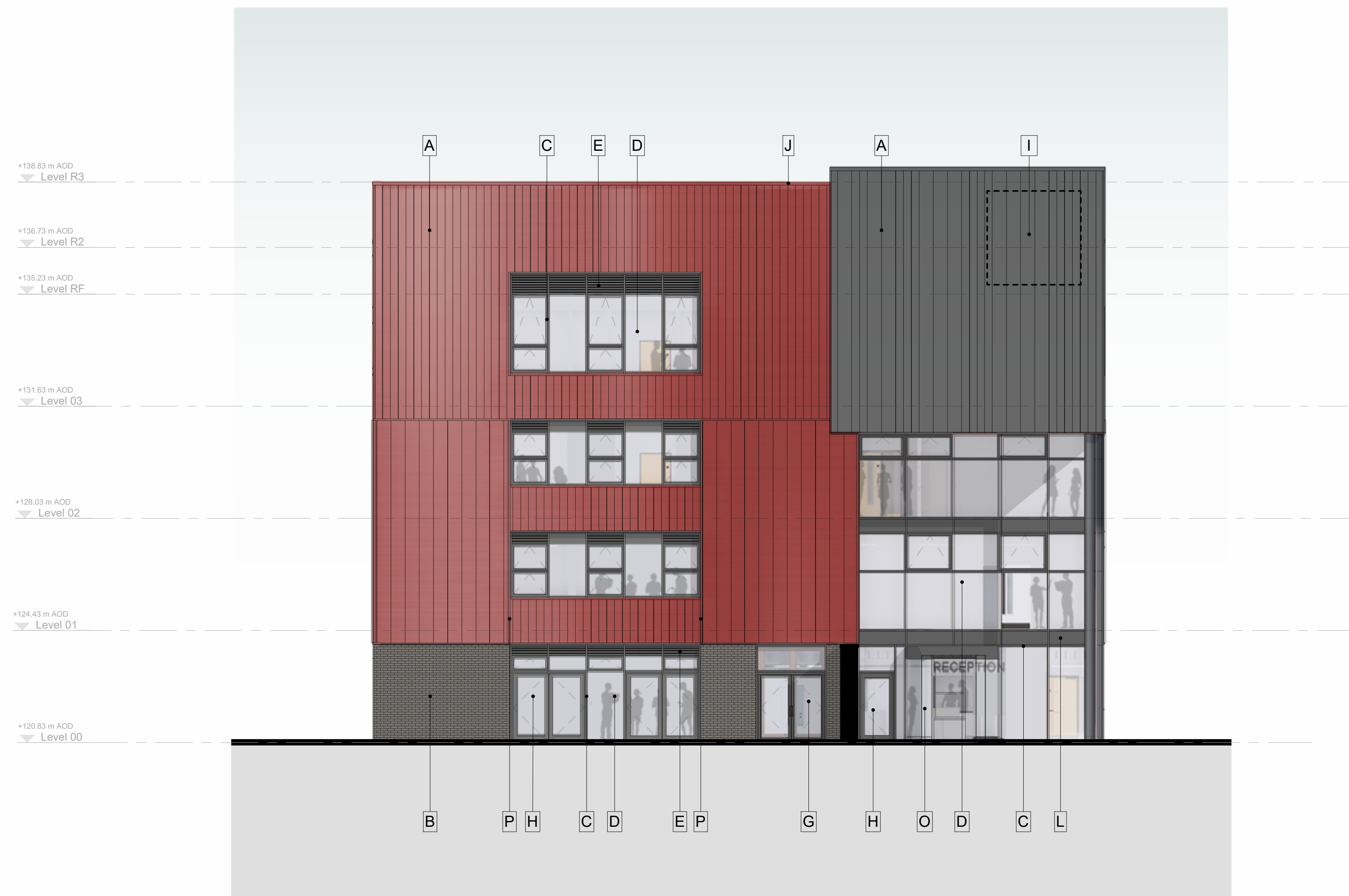
1 East Elevation 1 : 100
