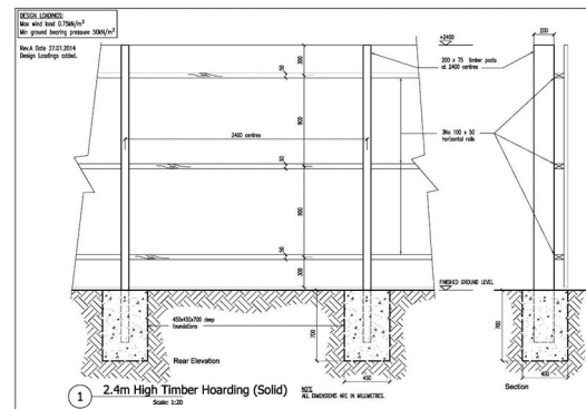
Figure 2 - Solid timber 2.4-metre-high hoarding
