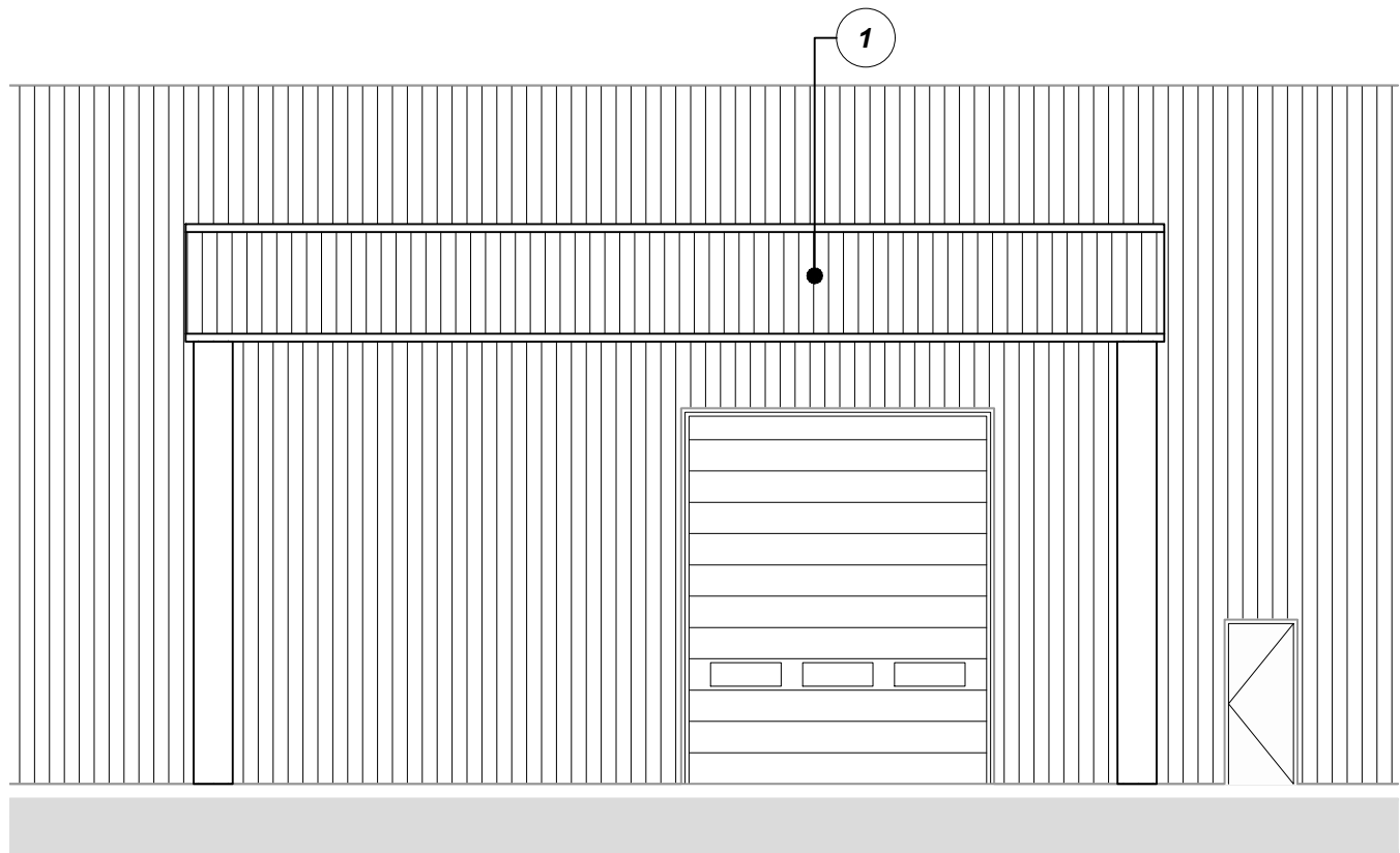
Canopy 2 - Eastern Elevation Scale 1:100
