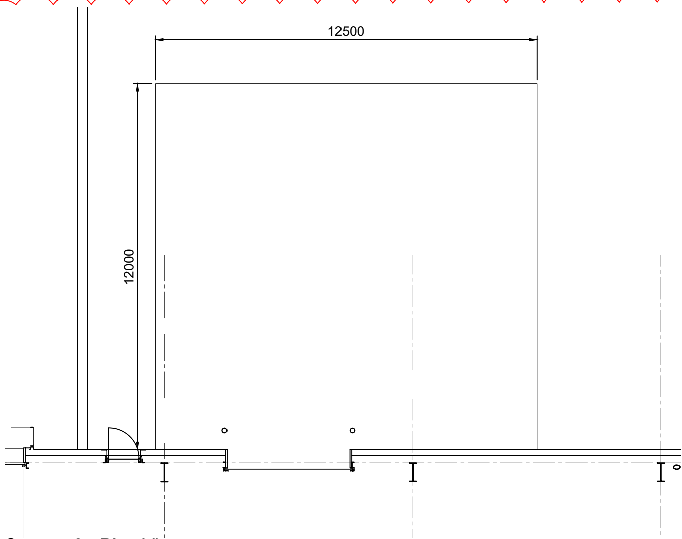
Canopy 2 - Plan View Scale 1:125
