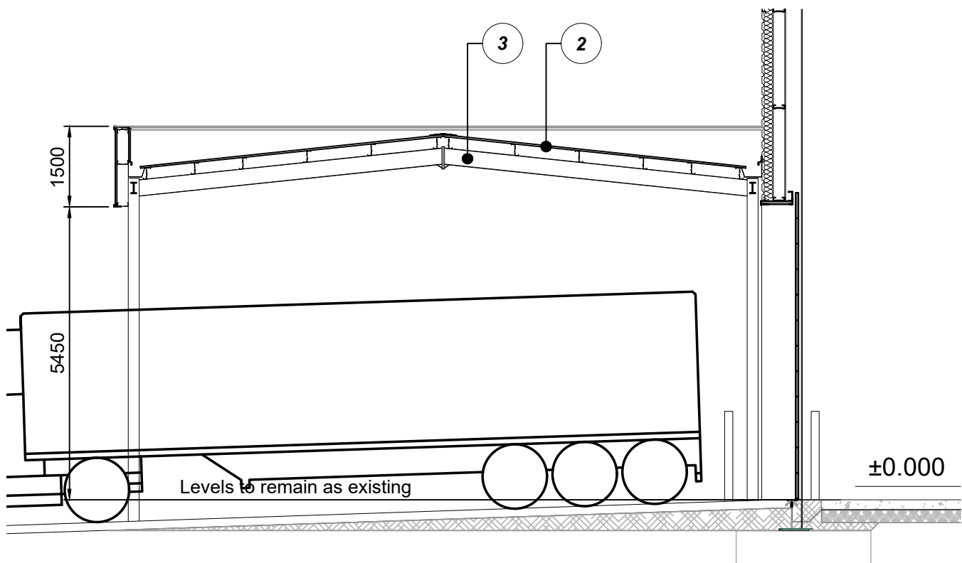
Typical Cut Thru Section Scale 1:100
