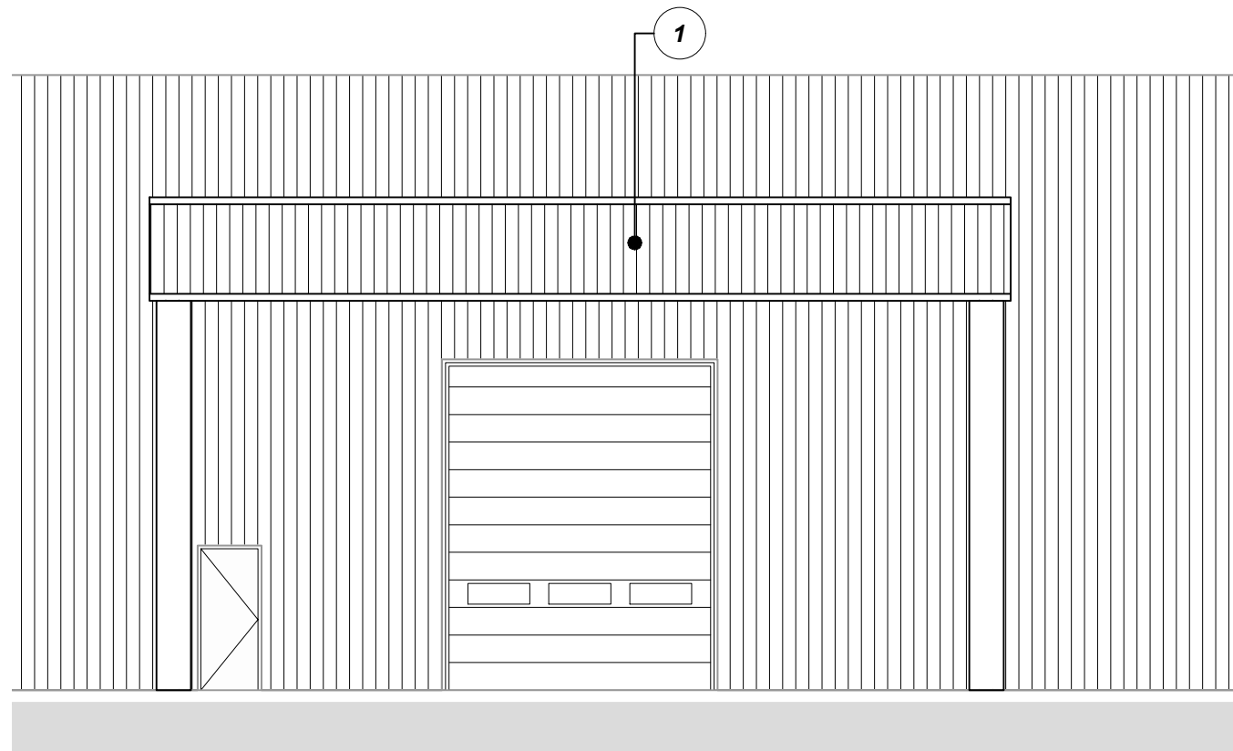
Canopy 1 - Eastern Elevation Scale 1:100
