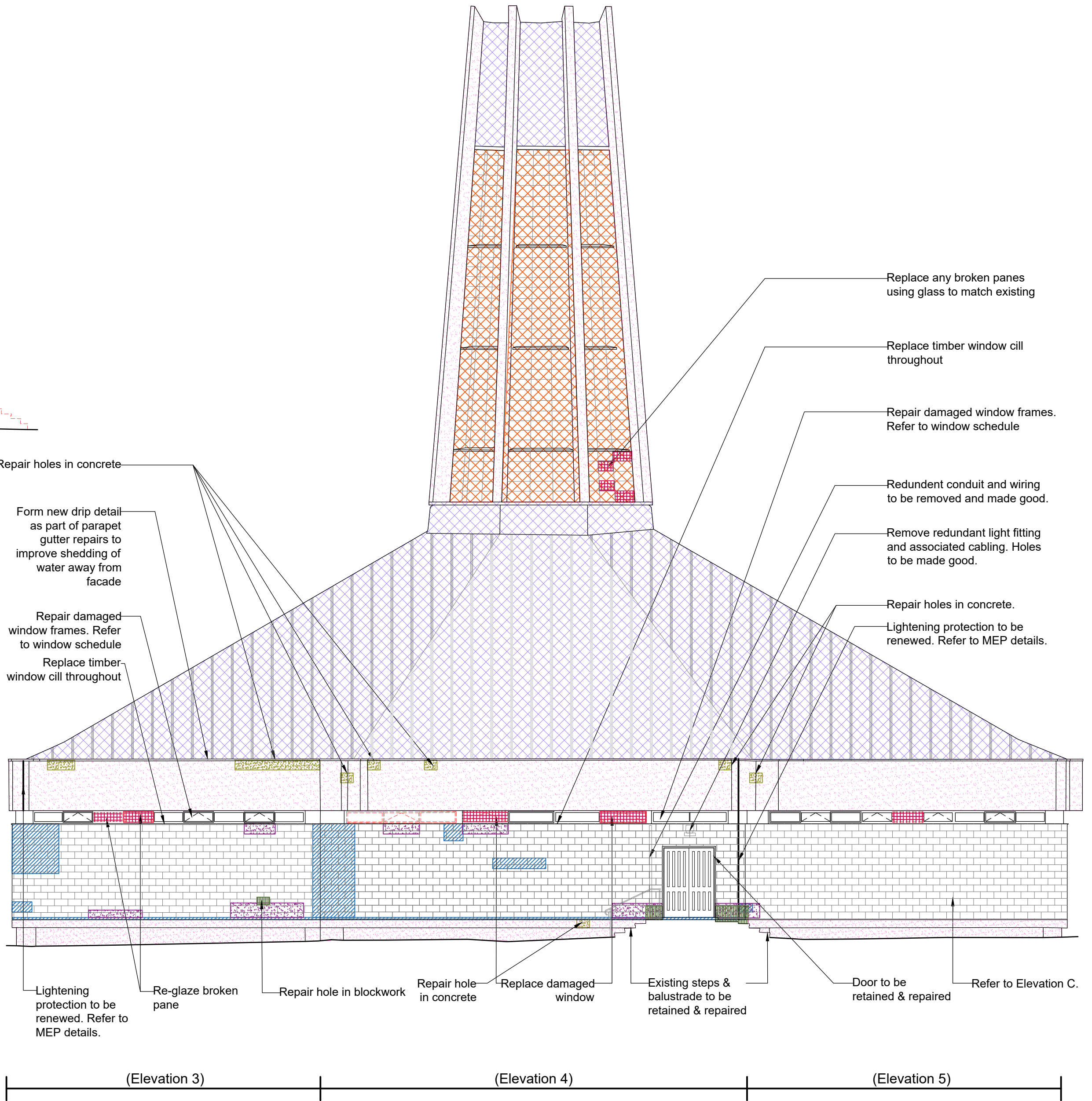
Elevation D
