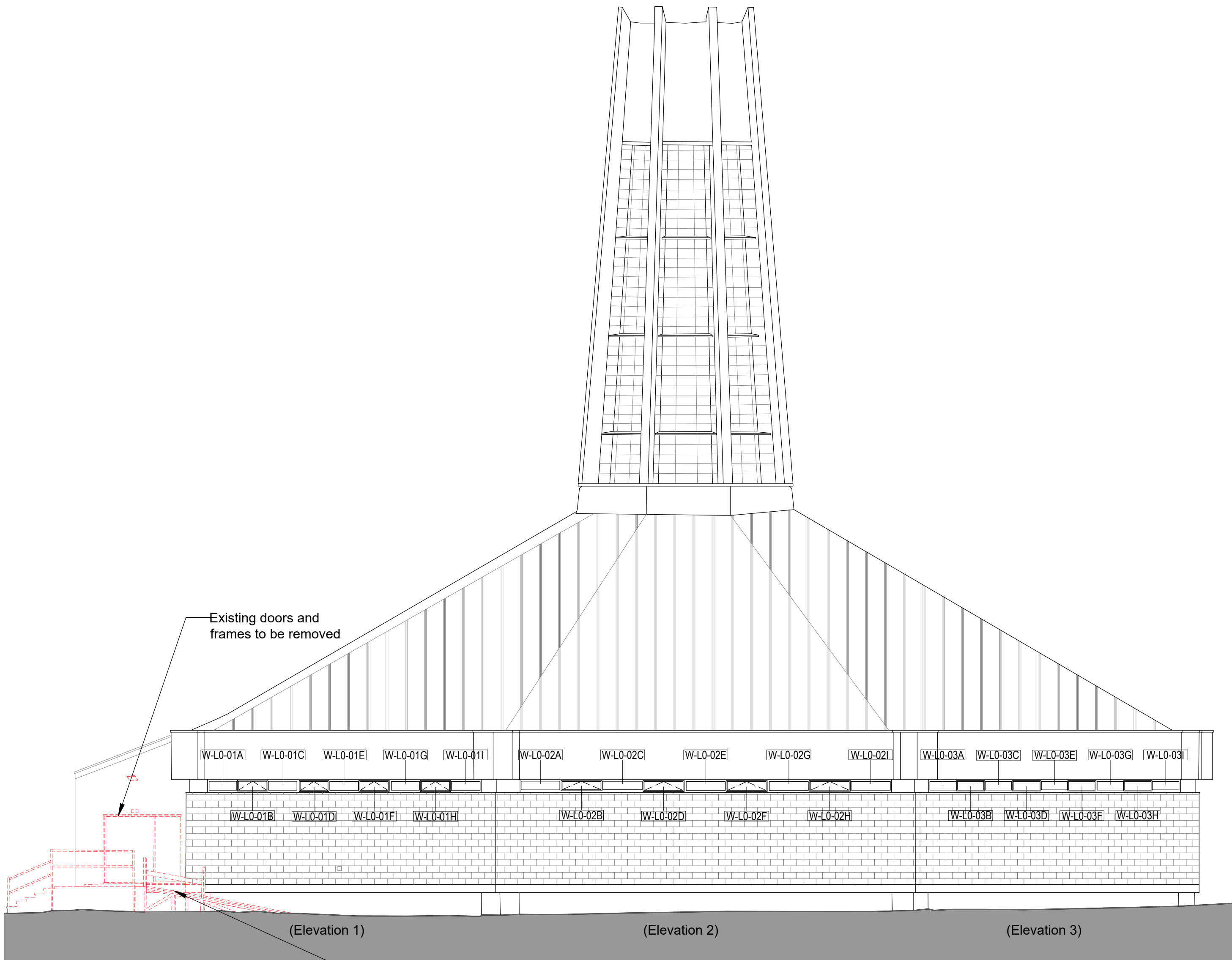
Existing Elevation B
