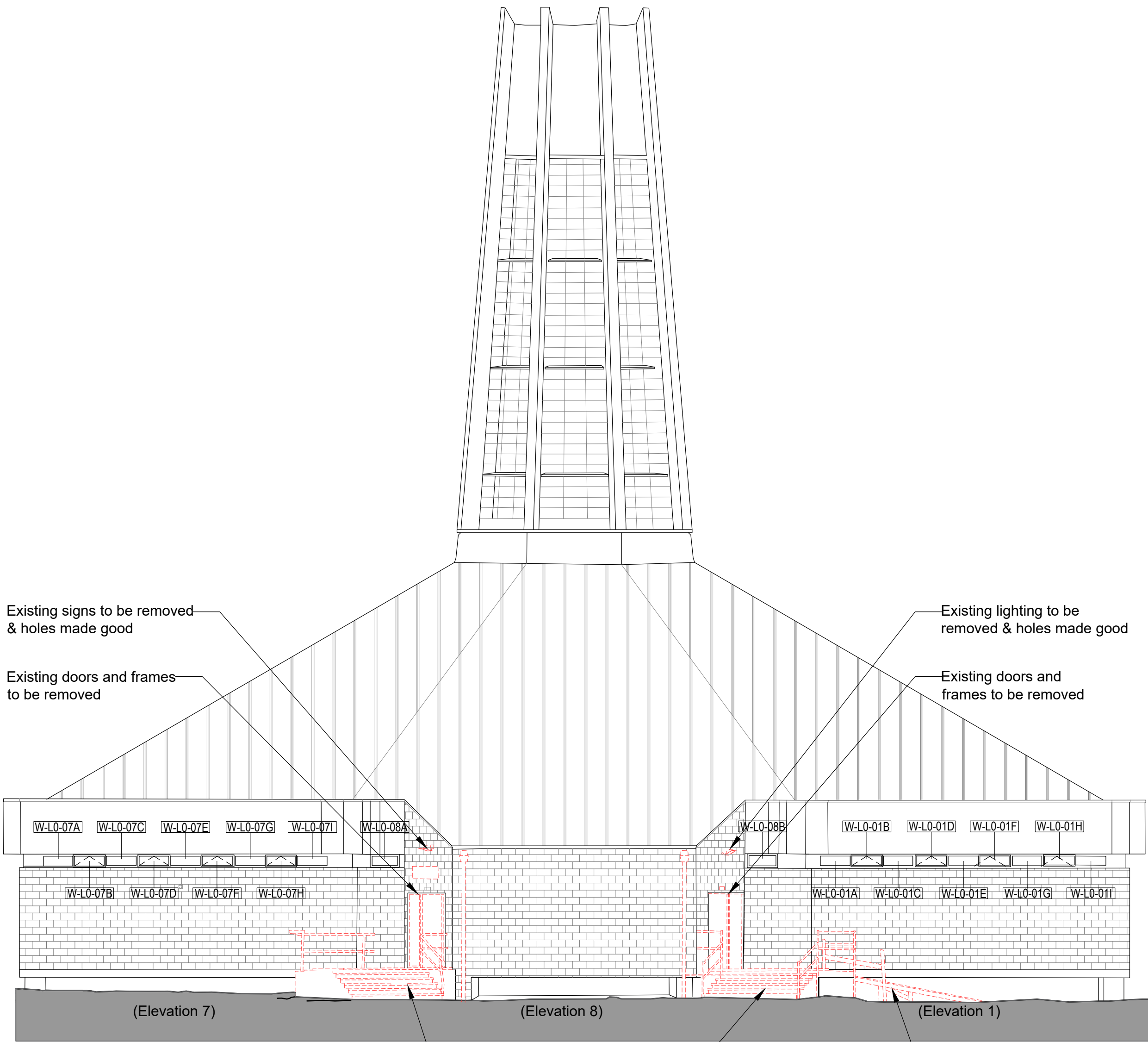
Existing Elevation A
