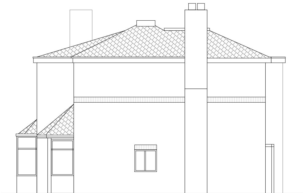
Existing Side Elevation(East) Scale - 1:100@A3
