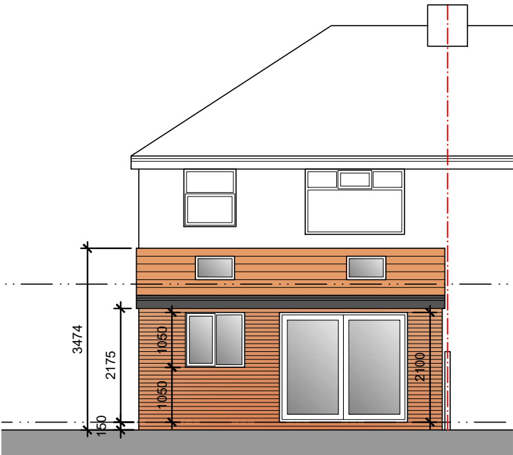
North Facing Rear Elevation
