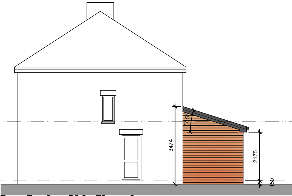
East Facing Side Elevation
