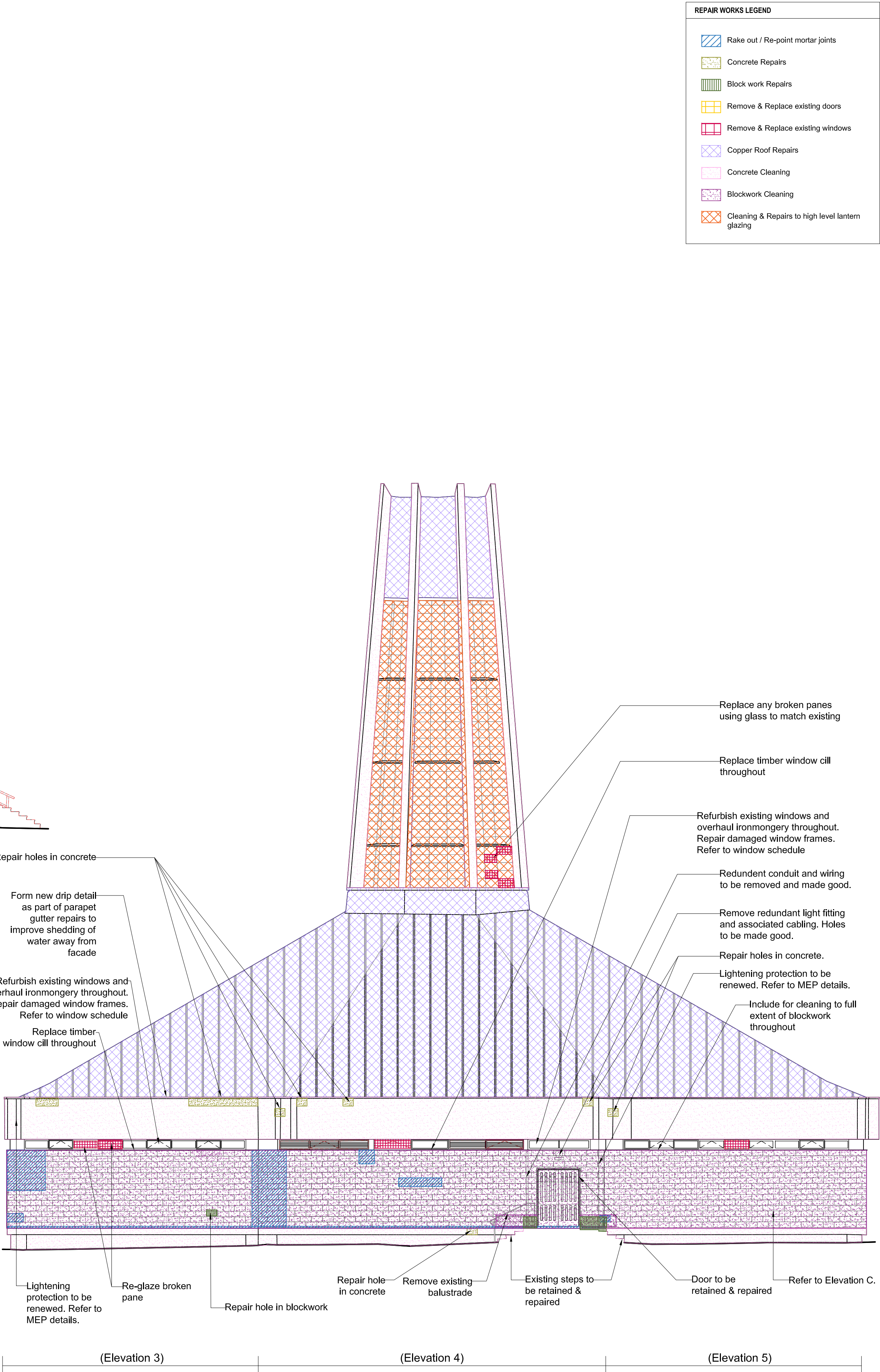
Elevation D
