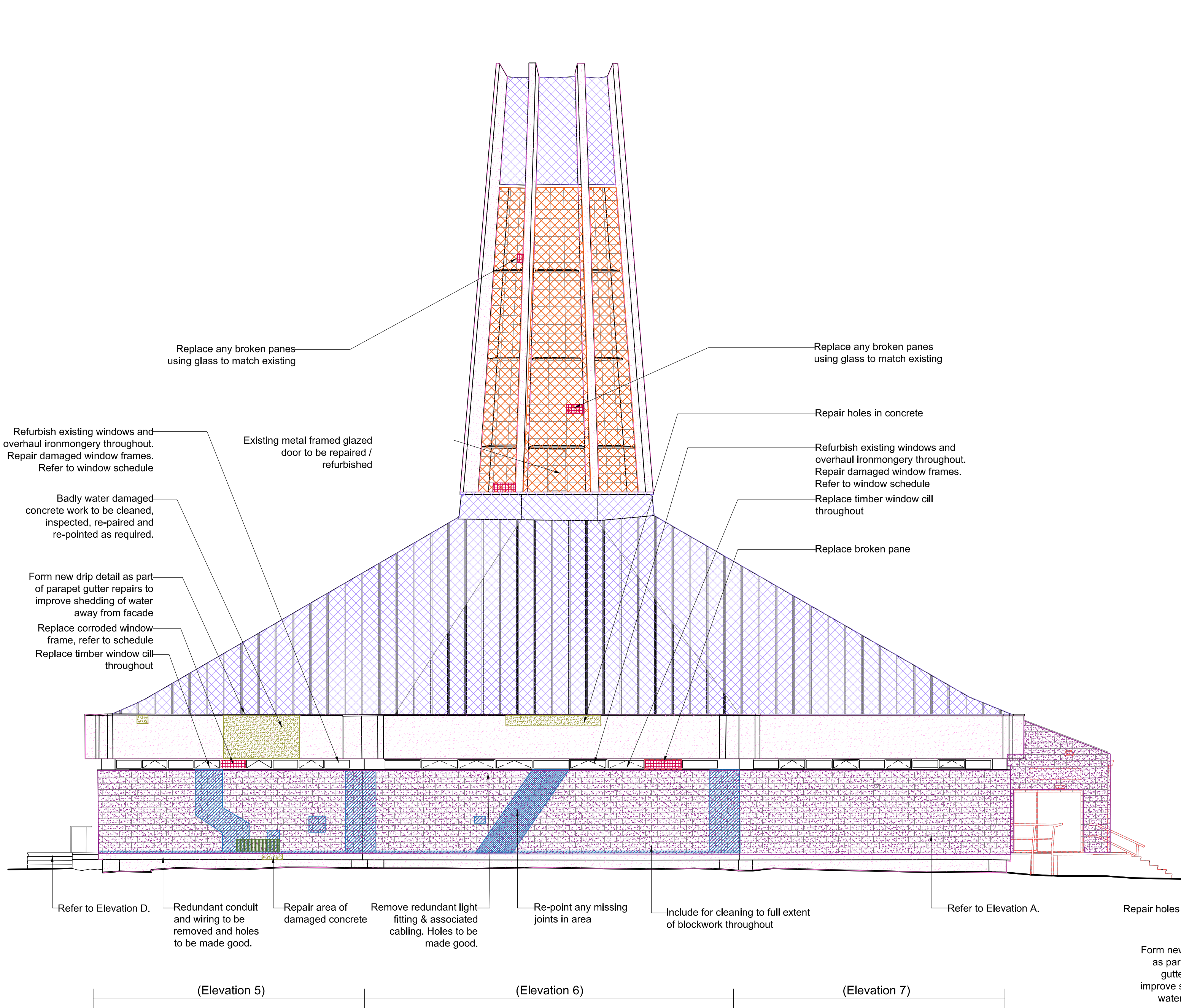
Elevation C
