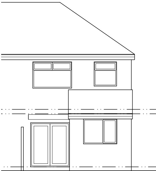
North Facing Rear Elevation
