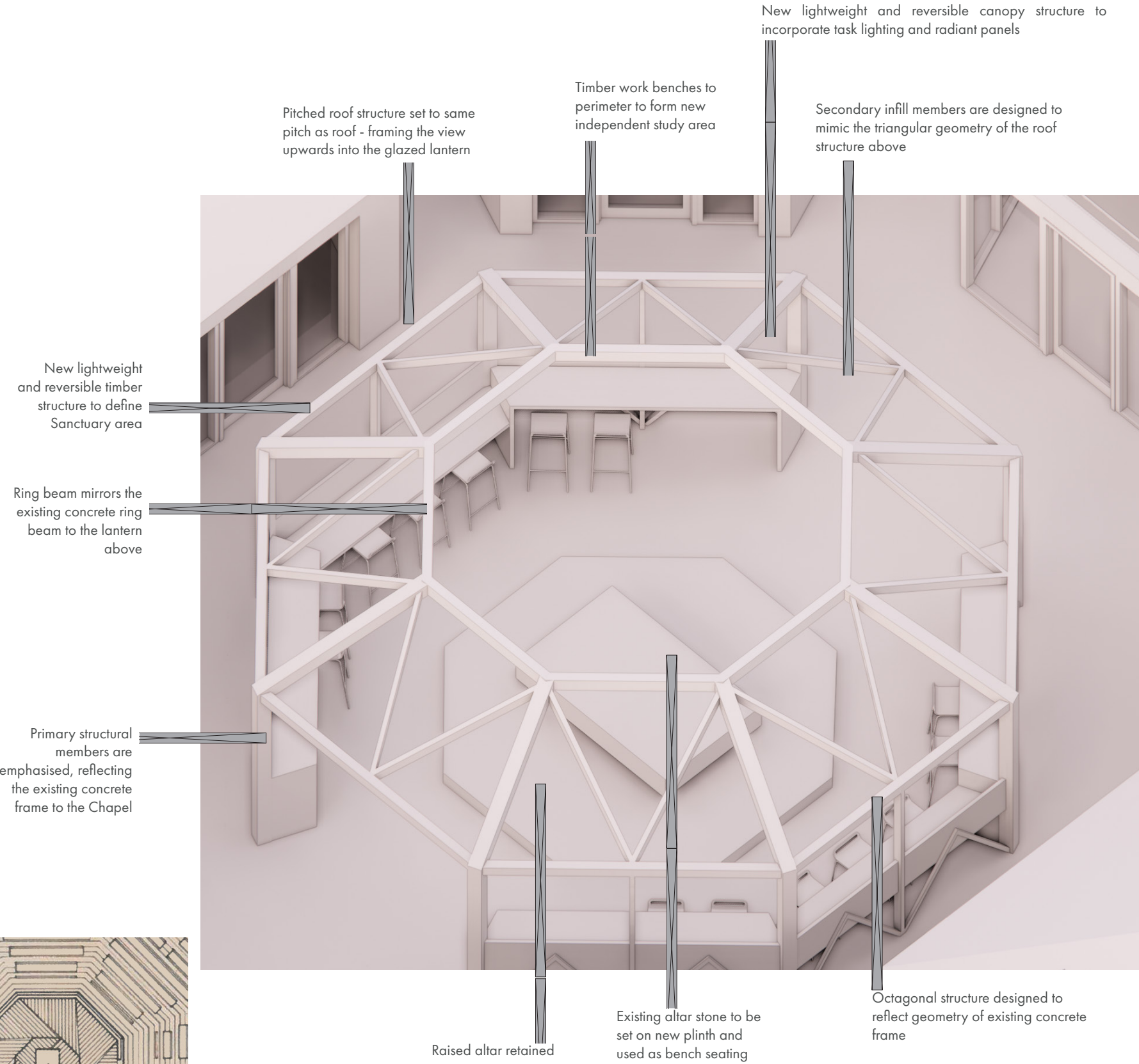
PROPOSED VIEW OF SANCTUARY AREA
