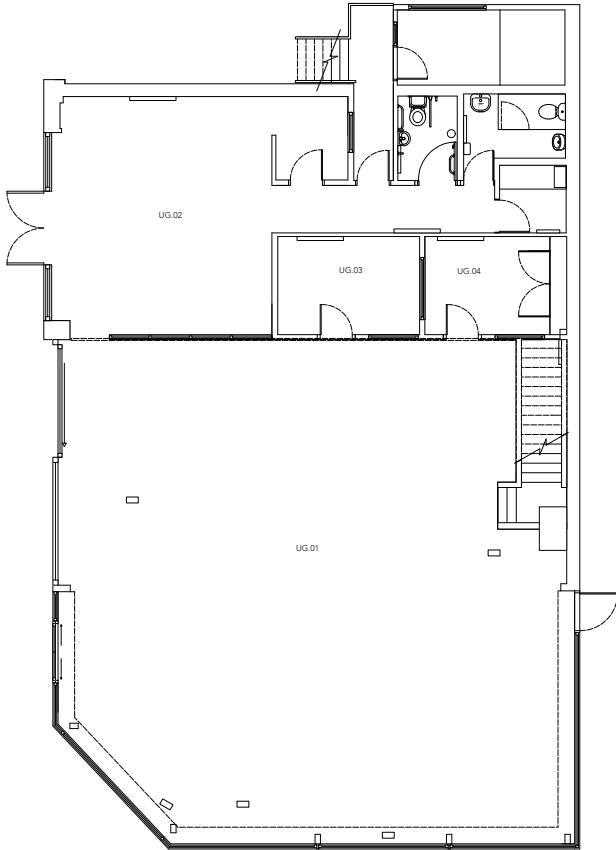
EXISTING UPPER GROUND GA
