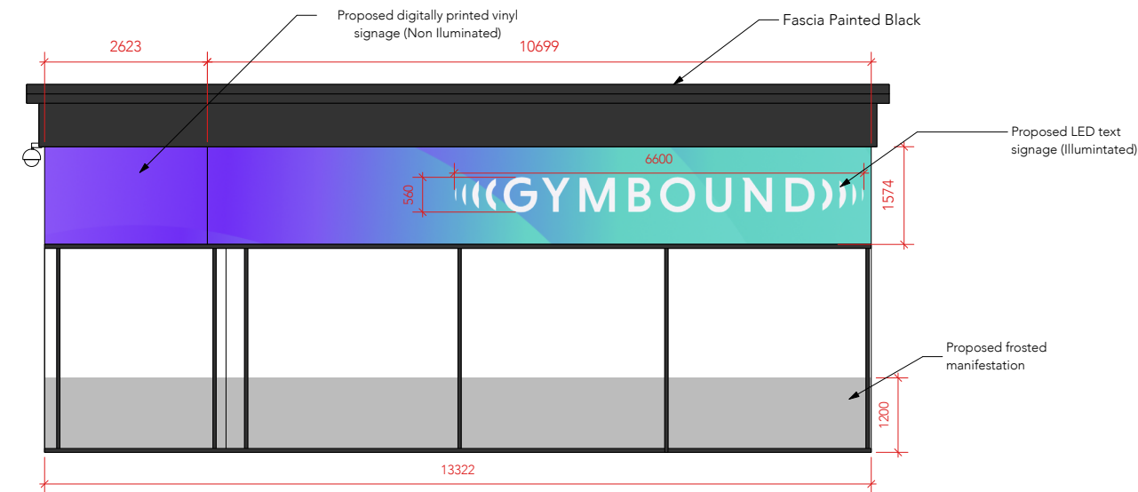
Splay Corner North West Elevation
