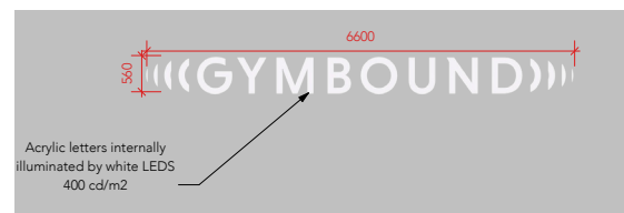
Signage Elevation
