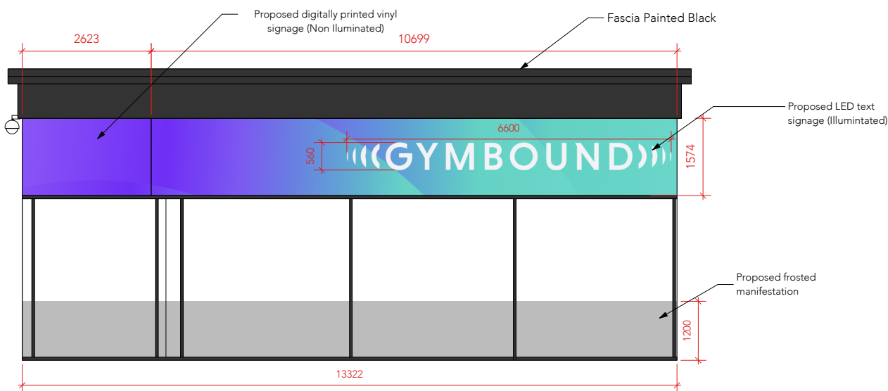
Splay Corner North West Elevation
