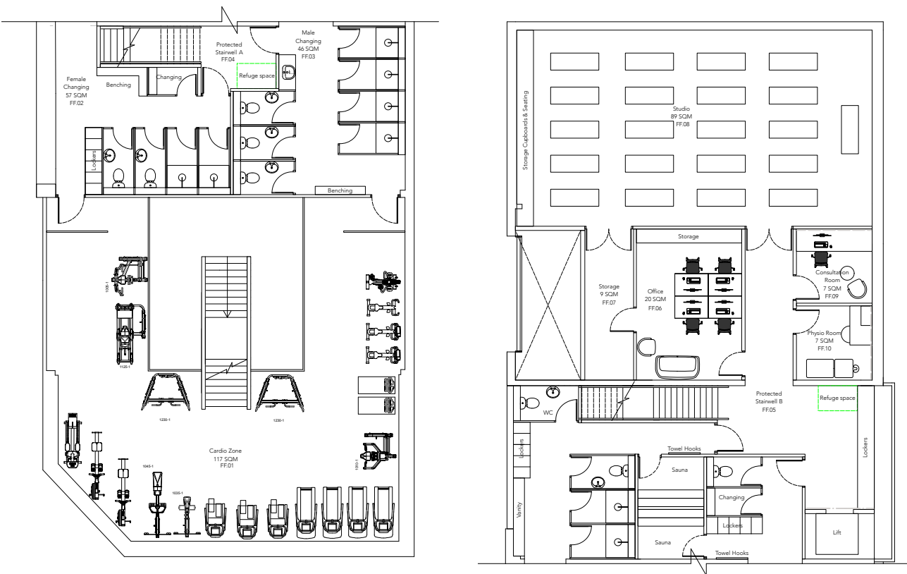
PROPOSED FIRST FLOOR GA
