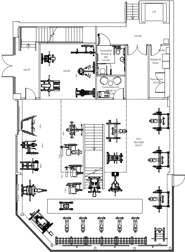
PROPOSED UPPER GROUND GA
