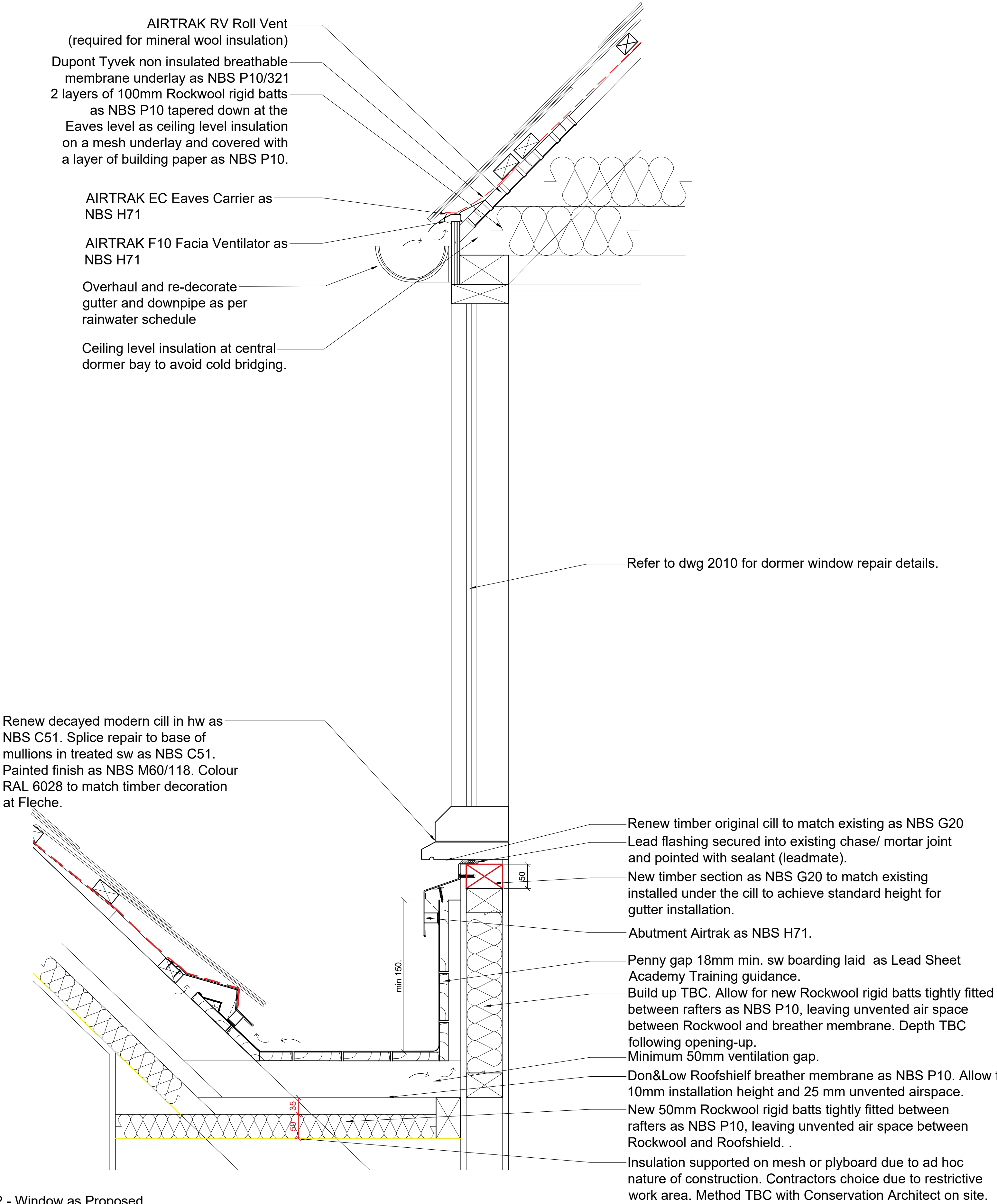
02 - Window as Proposed
