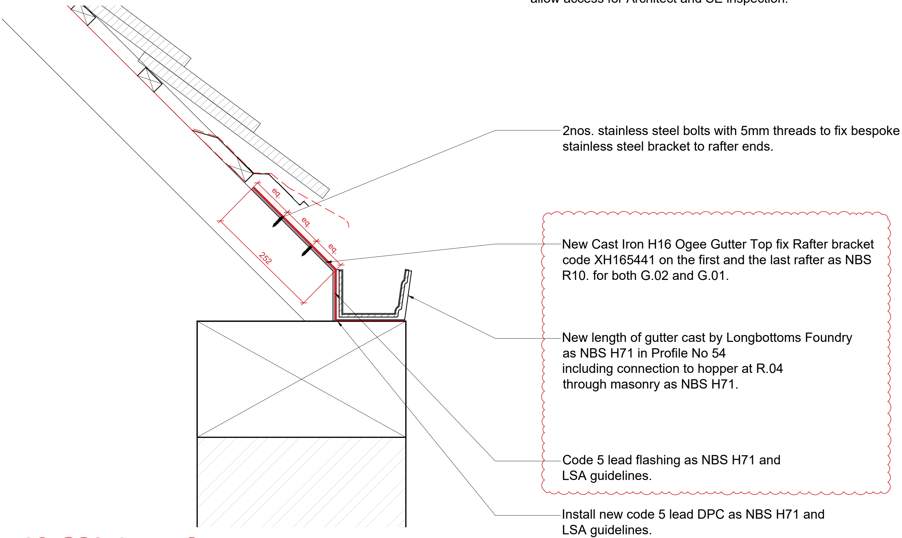
02 - Gutter G02 re-fixing detail.
