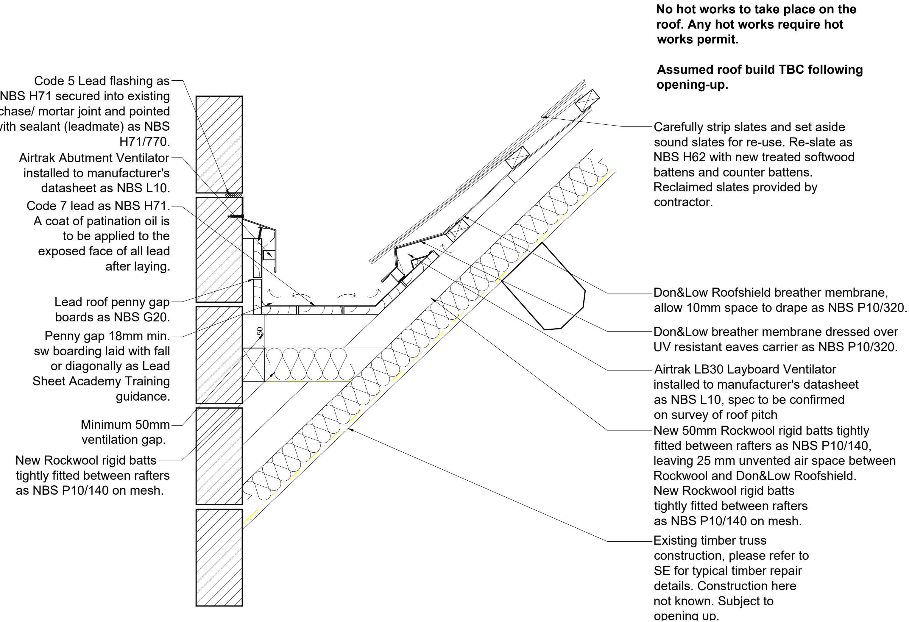
01 - Ventilated Eaves
