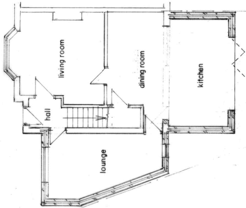
GROUND FLOOR PLAN (PROPOSED)
