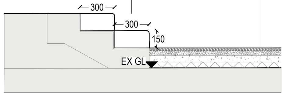
02 ST2 Yorkstone Steps Section Scale 1: 20 @A1
