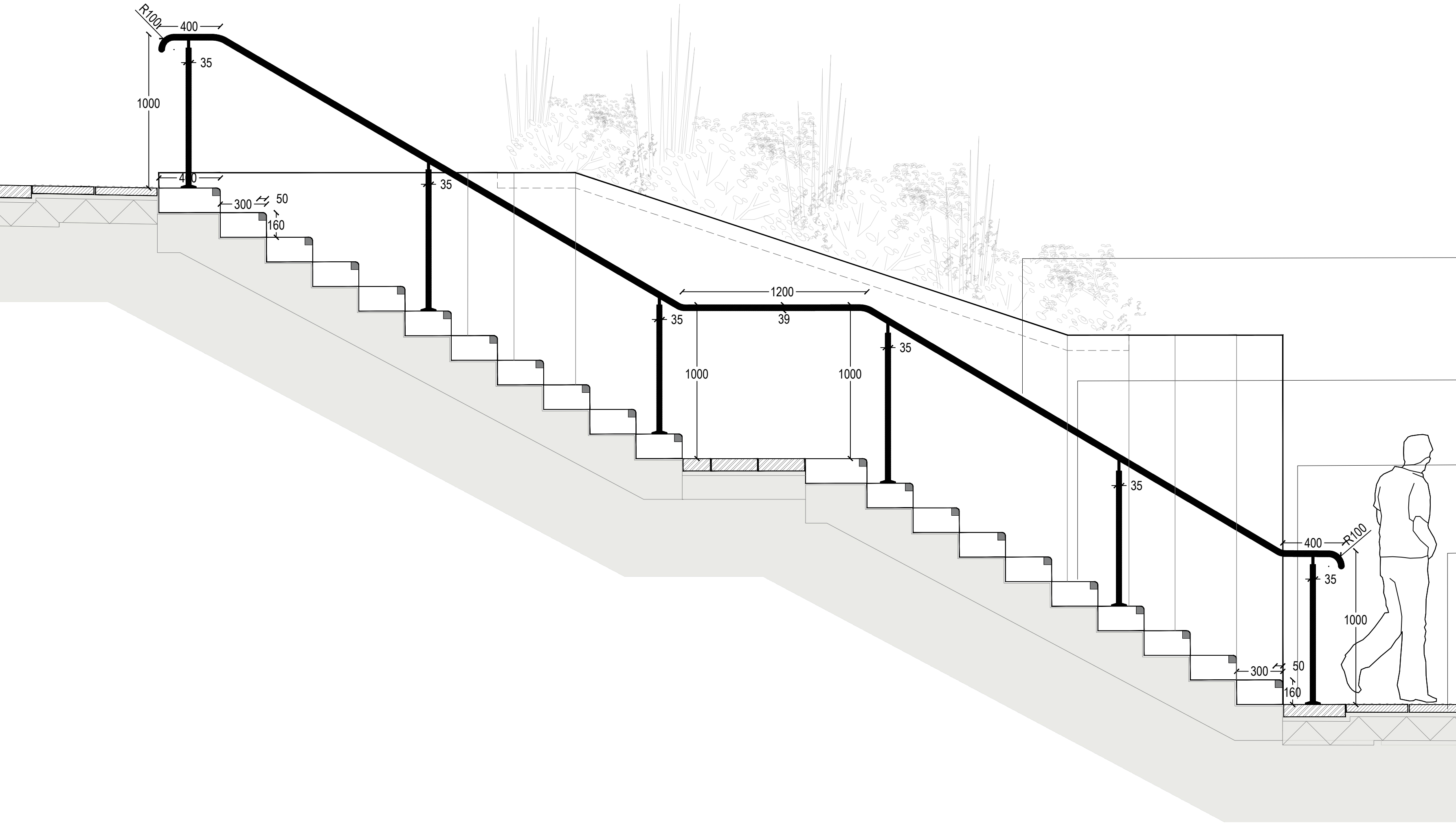
02 ST1 Yorkstone Steps Section A-A (Basement Access) Scale 1: 20 @A1
