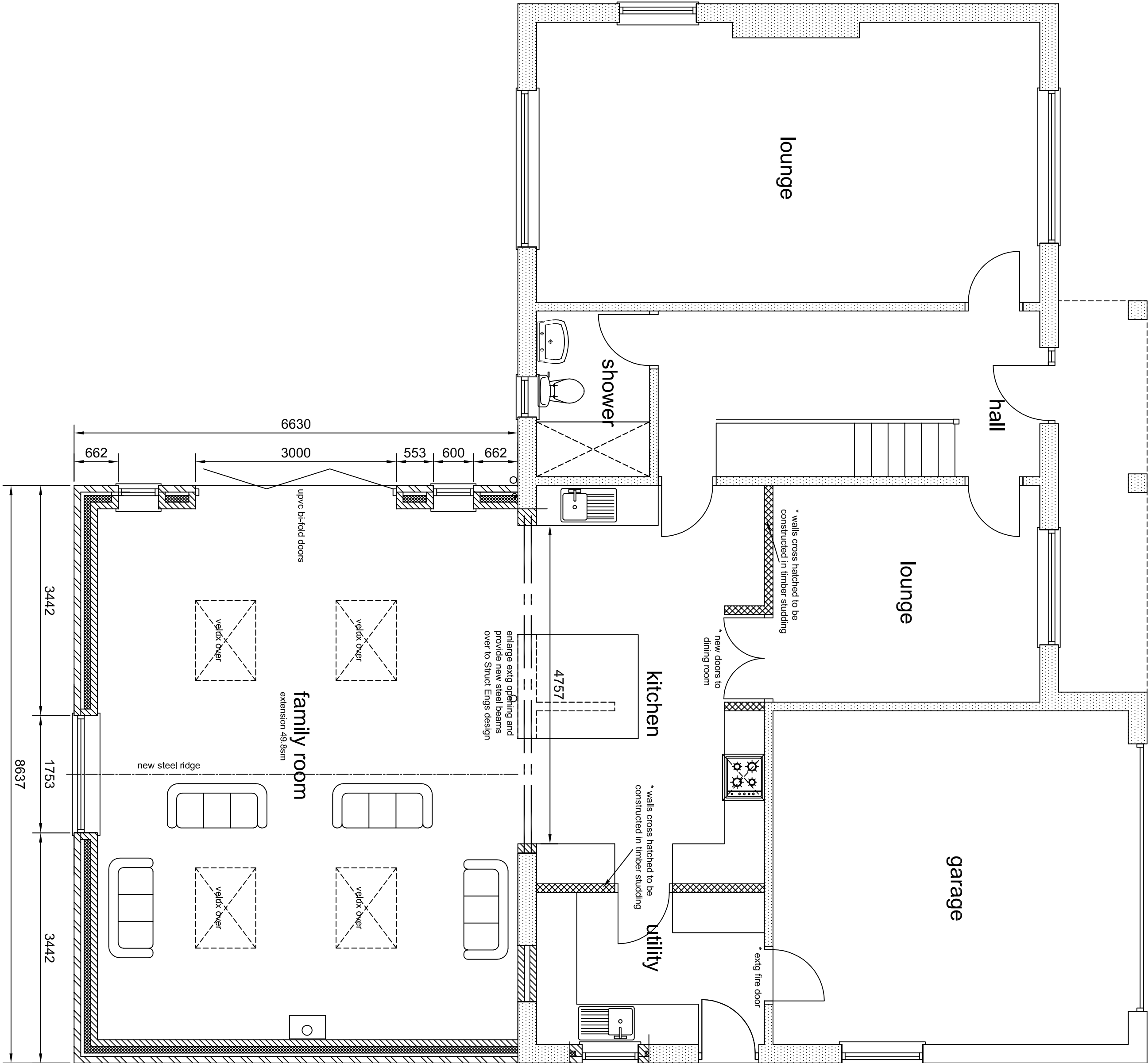
proposed overall ground floor
