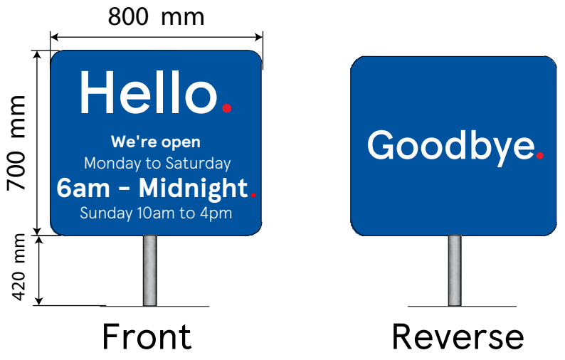
SIGN 7, 8 800 x1120 mm New pole mounted Hello/Goodbye sign to be installed. scale (1:20)
