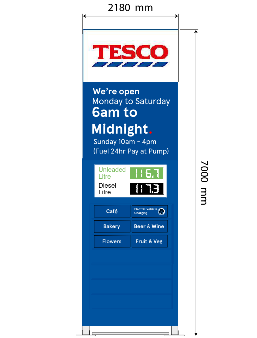
SIGN 4, 5 2180 x7000 mm Proposed 7m high internally illuminated double sided gantry sign scale (1:50)
