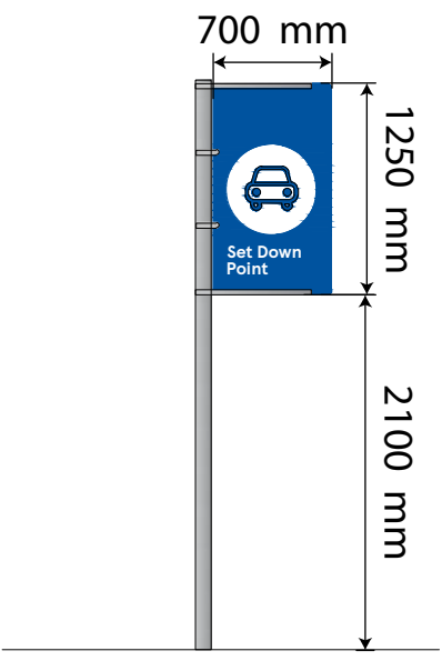
SIGN 6 700 x3350 mm New pole mounted Flag sign to installed scale (1:20)
