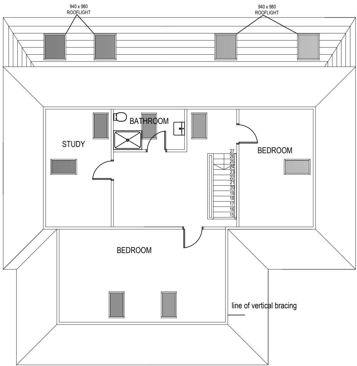
PROPOSED ATTIC PLAN
