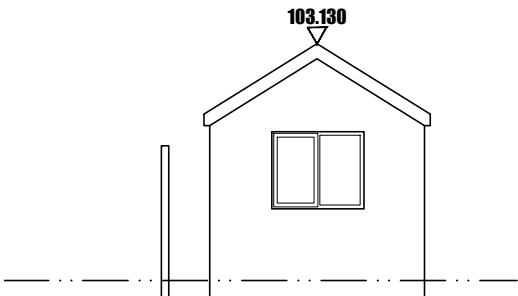
West Facing Side Elevation
