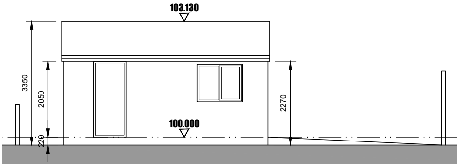
South Facing Front Elevation
