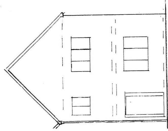
FRONT ELEVATION (EXISTING)
