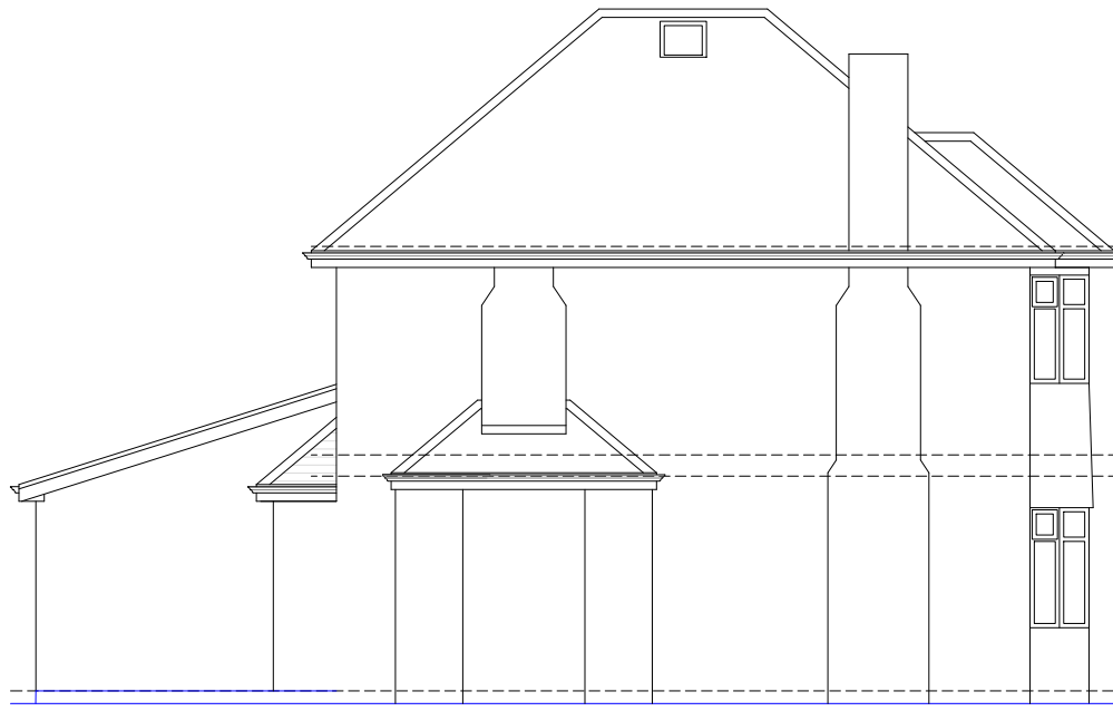
EXISTING SIDE ELEVATION (AS APPROVED)
