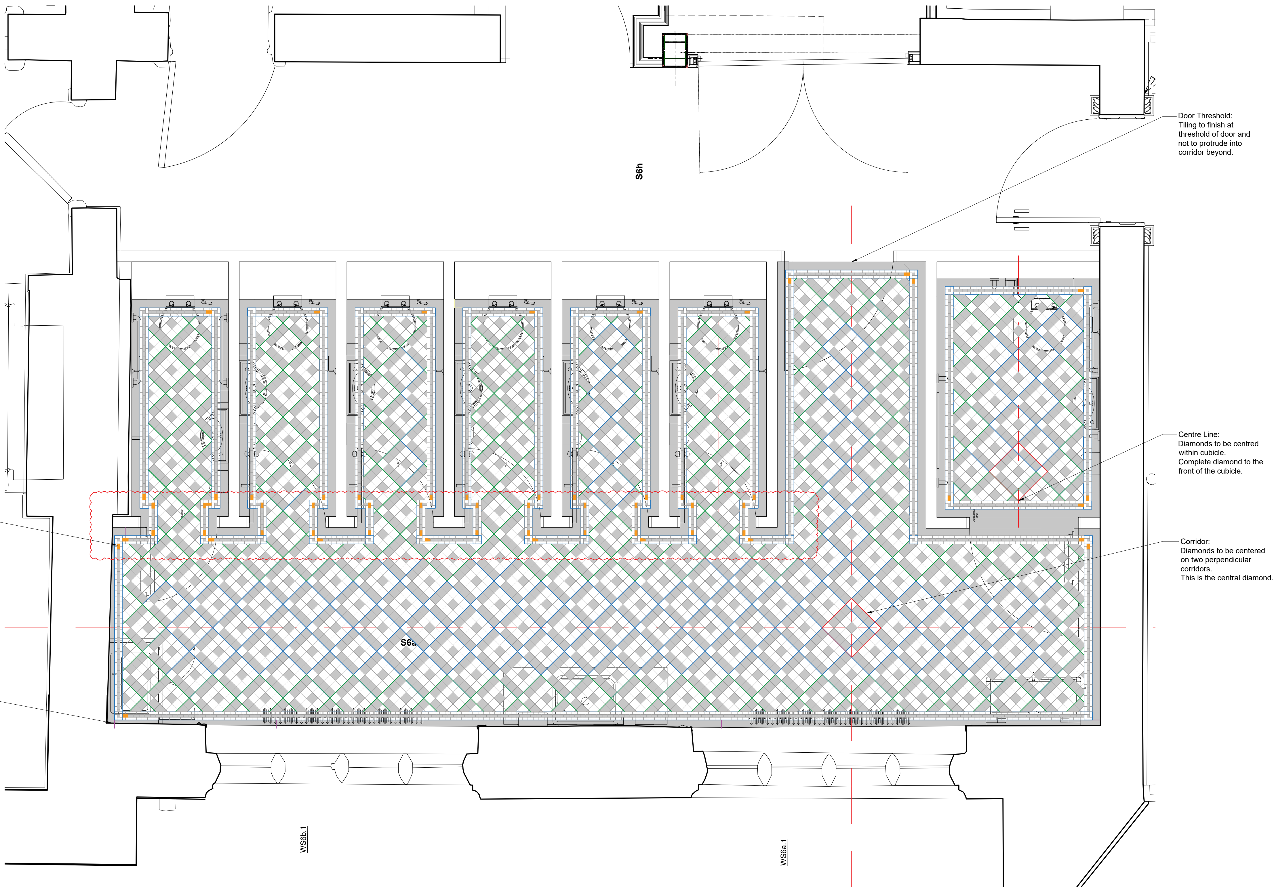
01 Second Floor WCs (All) - Karndean Layout 0086 Scale 1:20 @ A1
