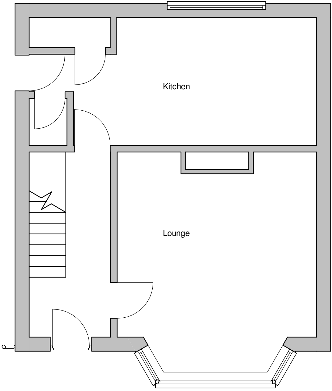
Existing Ground Floor 1 : 50
