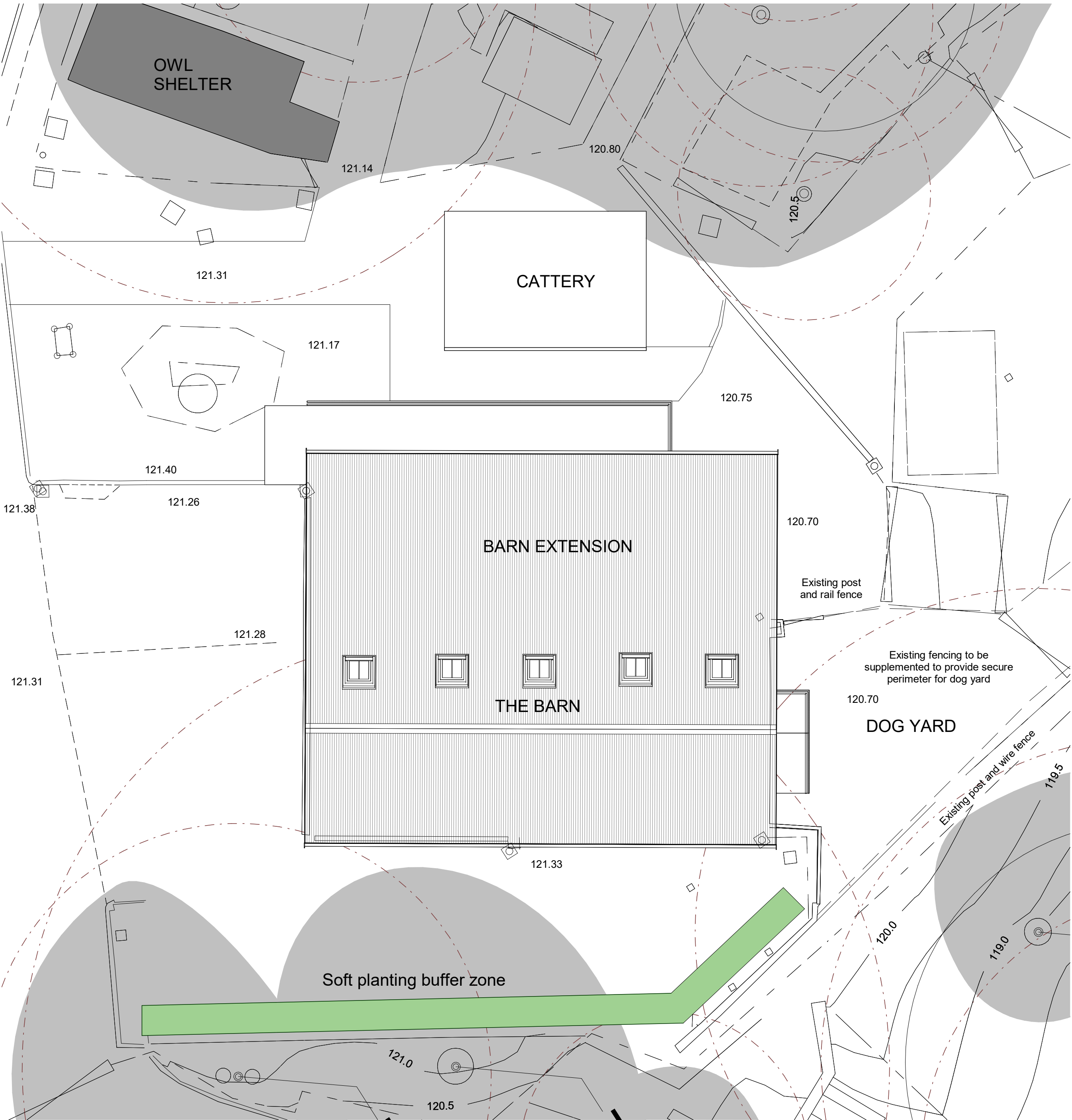
Barn Proposed Roofplan
