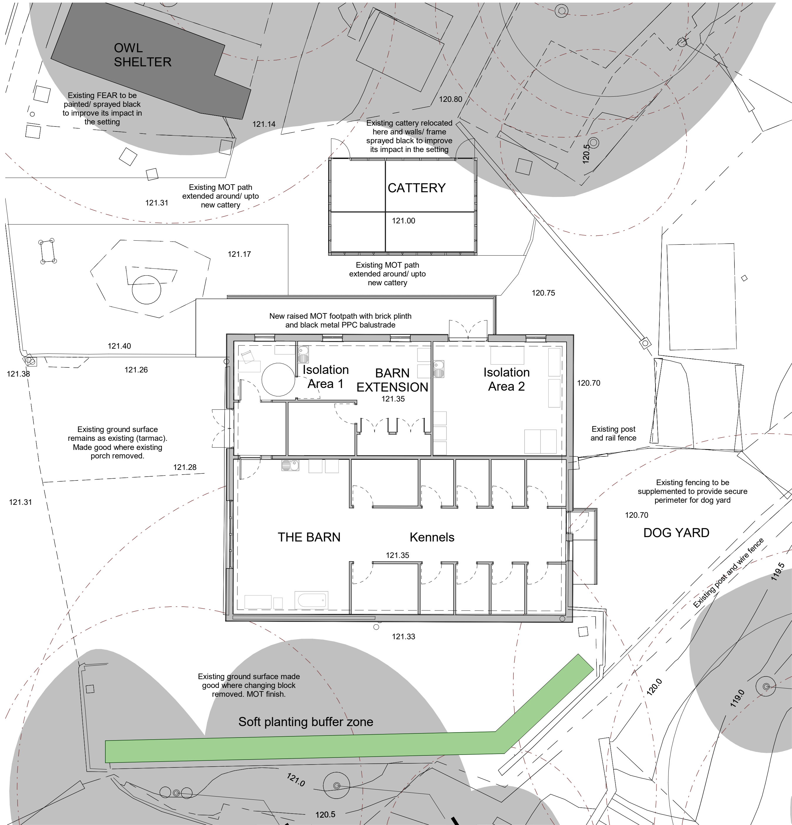
Barn Proposed Floorplan
