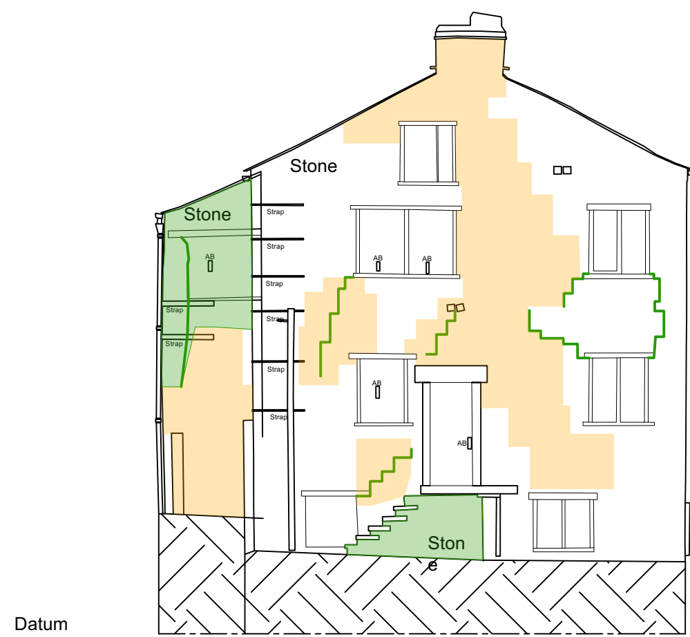
Elevation C
