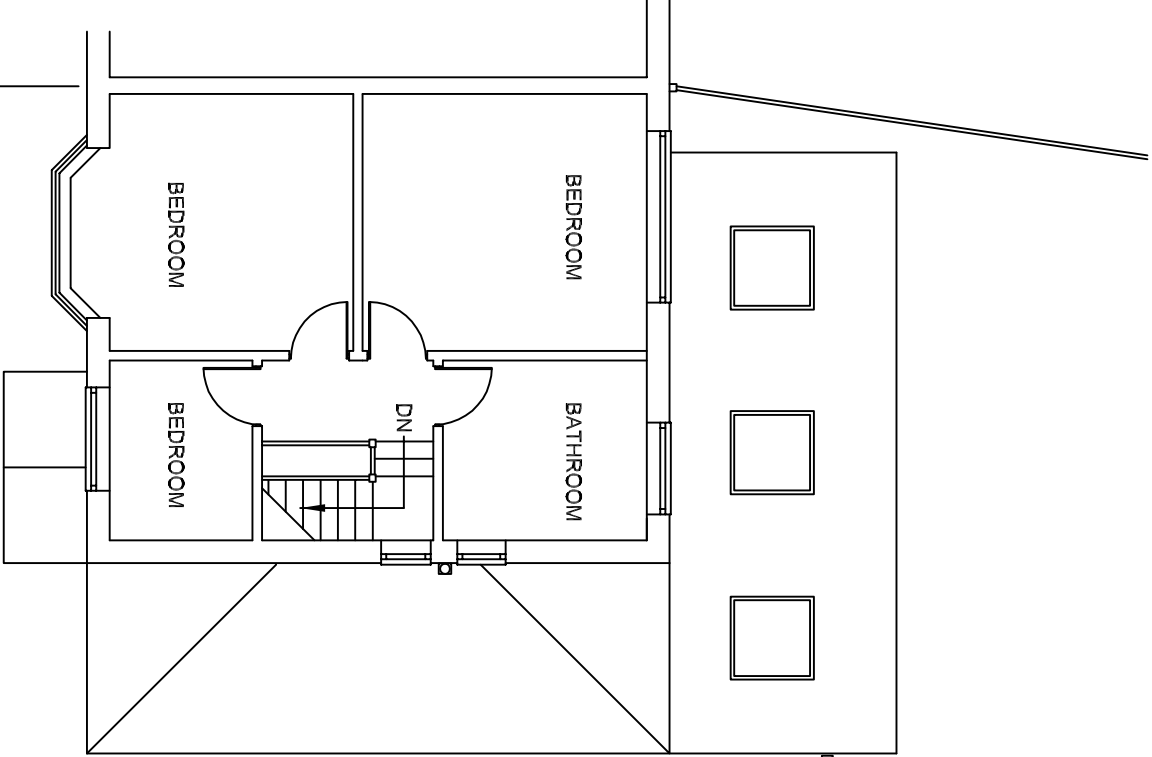
EXISTING F/F PLAN
