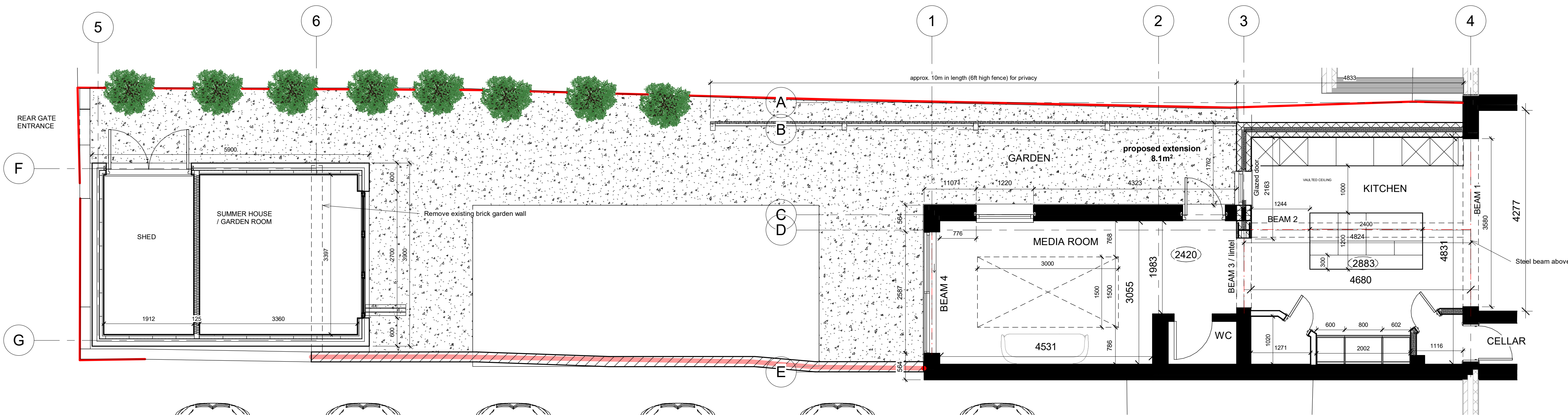
3 Proposed Garden 1 : 50
