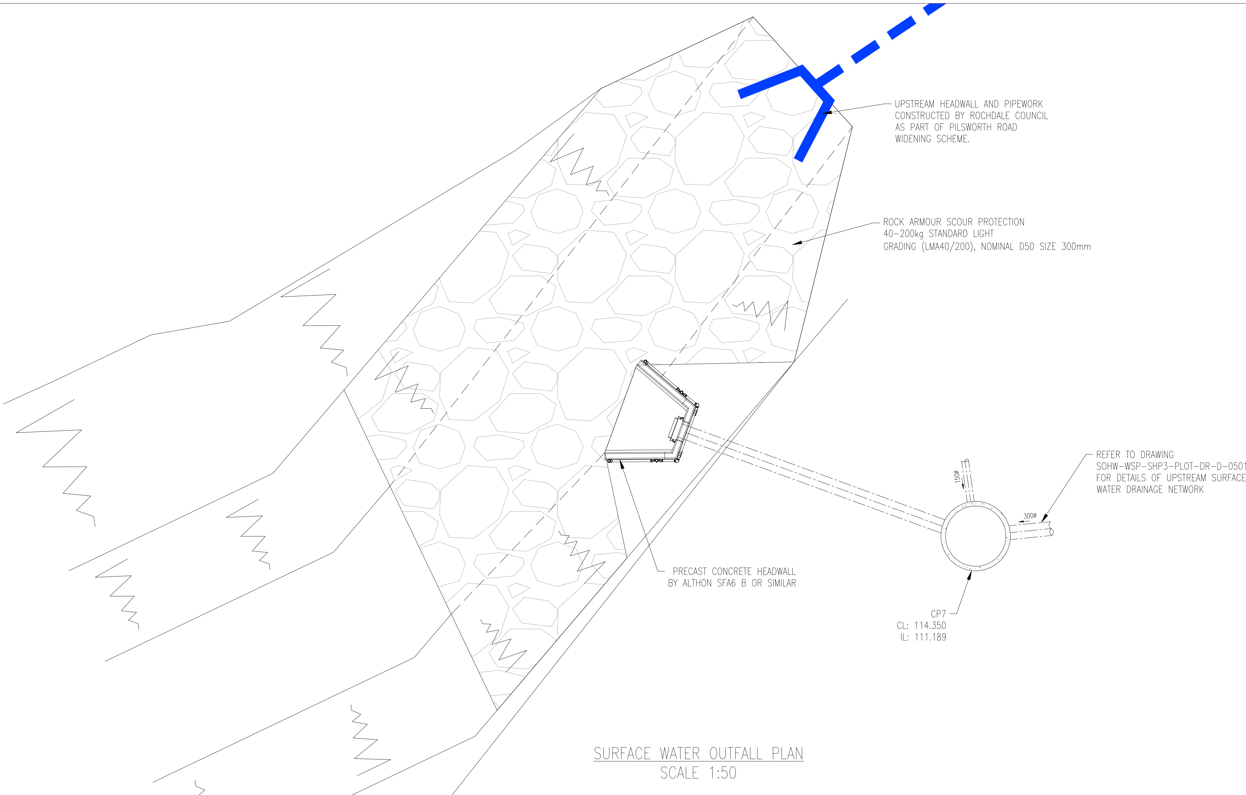
SURFACE WATER OUTFALL SECTION SCALE 1:50
