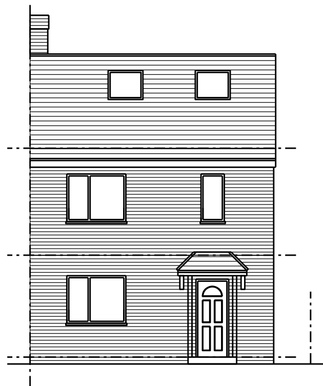
North Elevation
