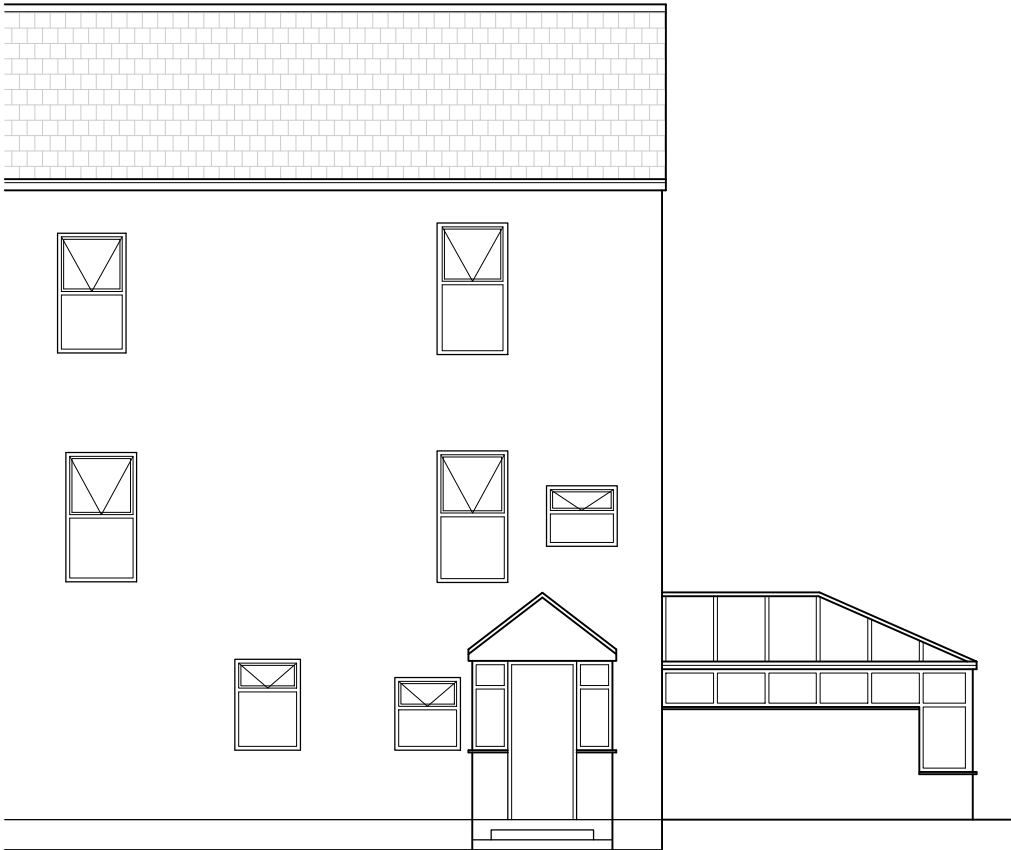
EXISTING FRONT ELEVATION 1:100 @ A3
