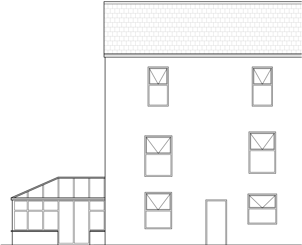
EXISTING REAR ELEVATION 1:100 @ A3
