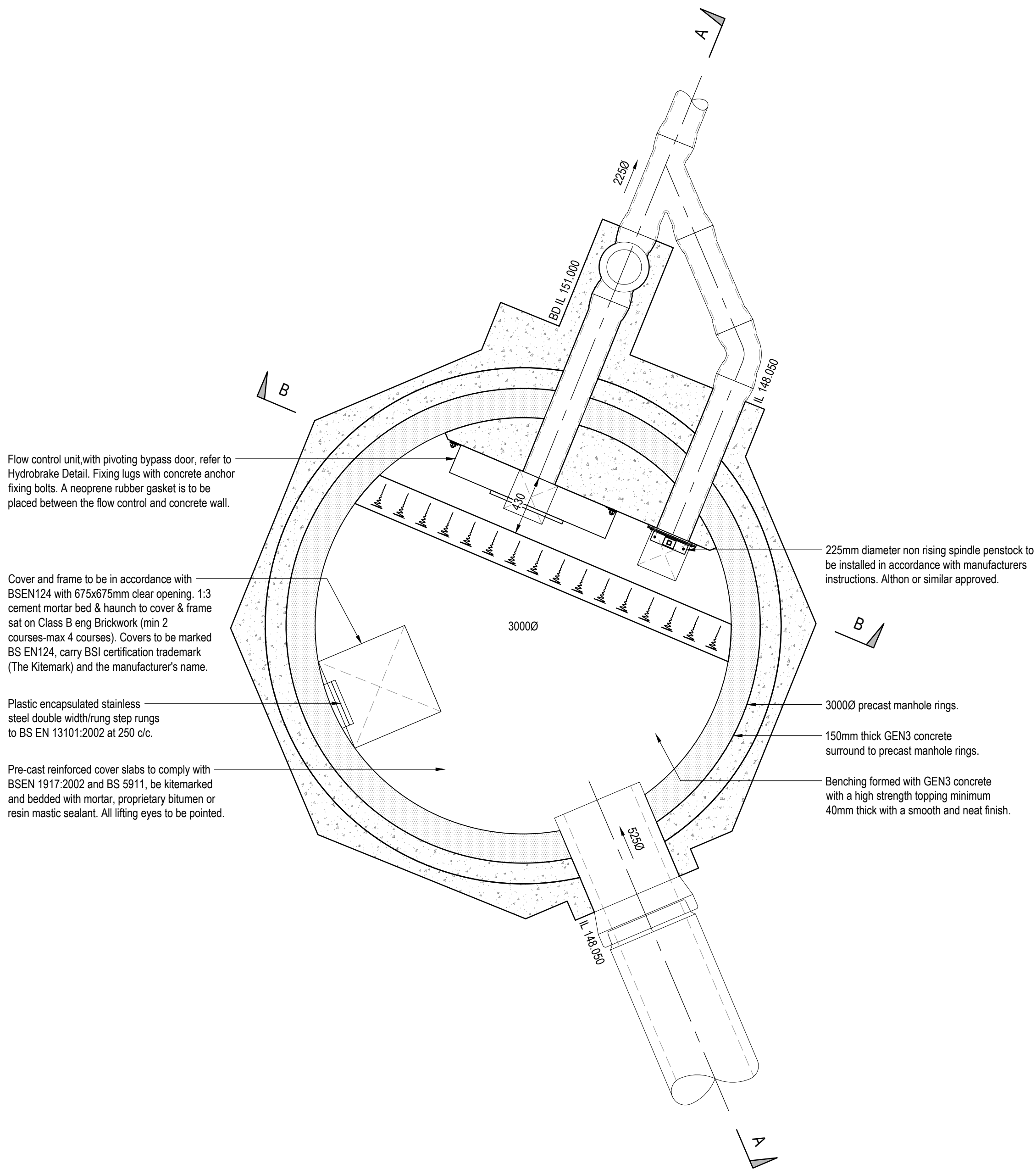
PLAN ON HYDROBRAKE MANHOLE S33
