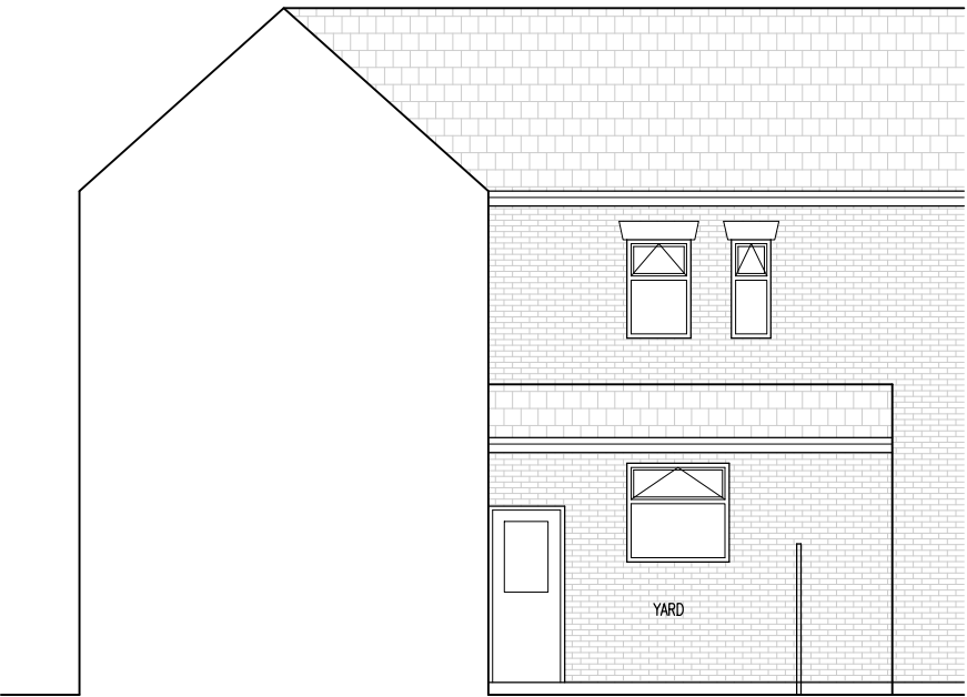
EXISTING ELEVATION (REAR) 1:100 @ A3
