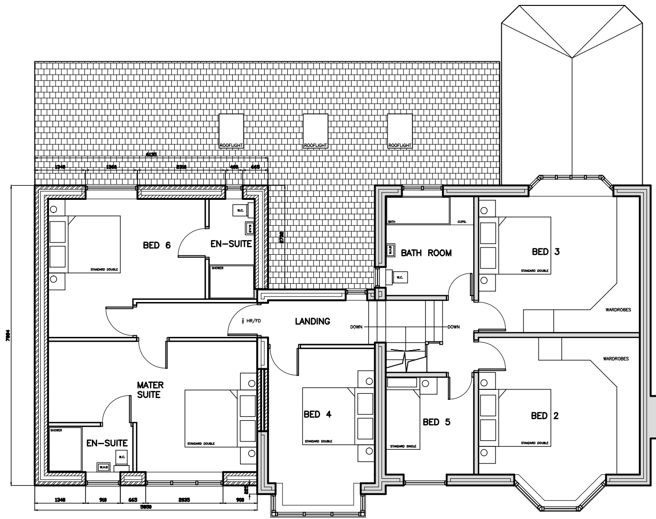
PROPOSED FIRST FLOOR LEVEL
